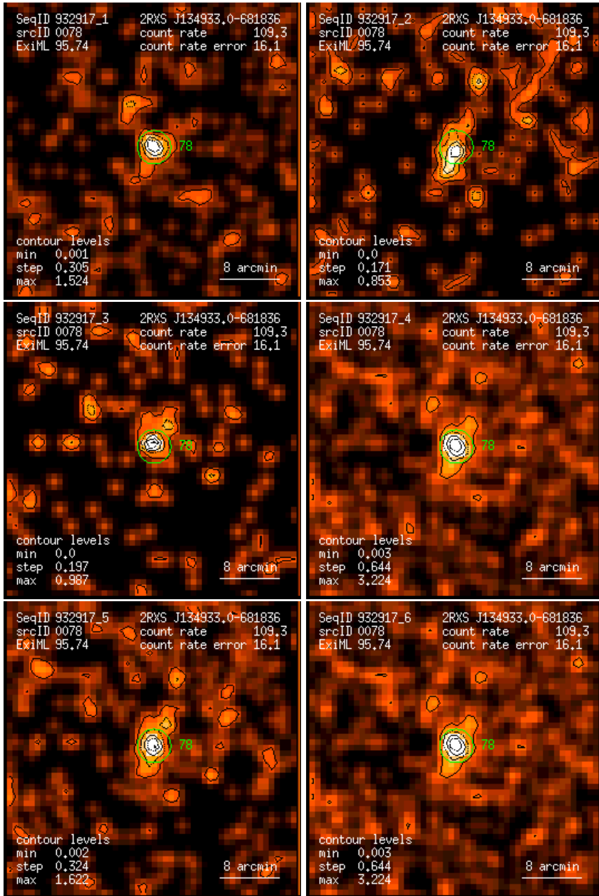
Figure 78: RASS 932917: detection 0078: band rate images, Gaussian filter: (1) PSPC channels 11 – 41, (2) 52 – 90, (3) 91 – 201, (4) 11 – 235, (5) 52 – 201, (6) 11 – 201. Broad band rates in counts/ks. Band rate contour levels in counts/ks/arcmin 2 .
