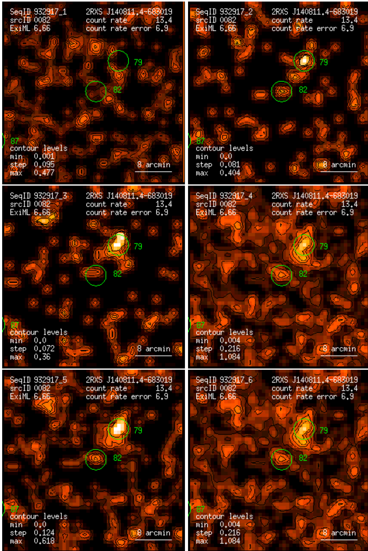
Figure 82: RASS 932917: detection 0082: band rate images, Gaussian filter: (1) PSPC channels 11 – 41, (2) 52 – 90, (3) 91 – 201, (4) 11 – 235, (5) 52 – 201, (6) 11 – 201. Broad band rates in counts/ks. Band rate contour levels in counts/ks/arcmin 2 .
