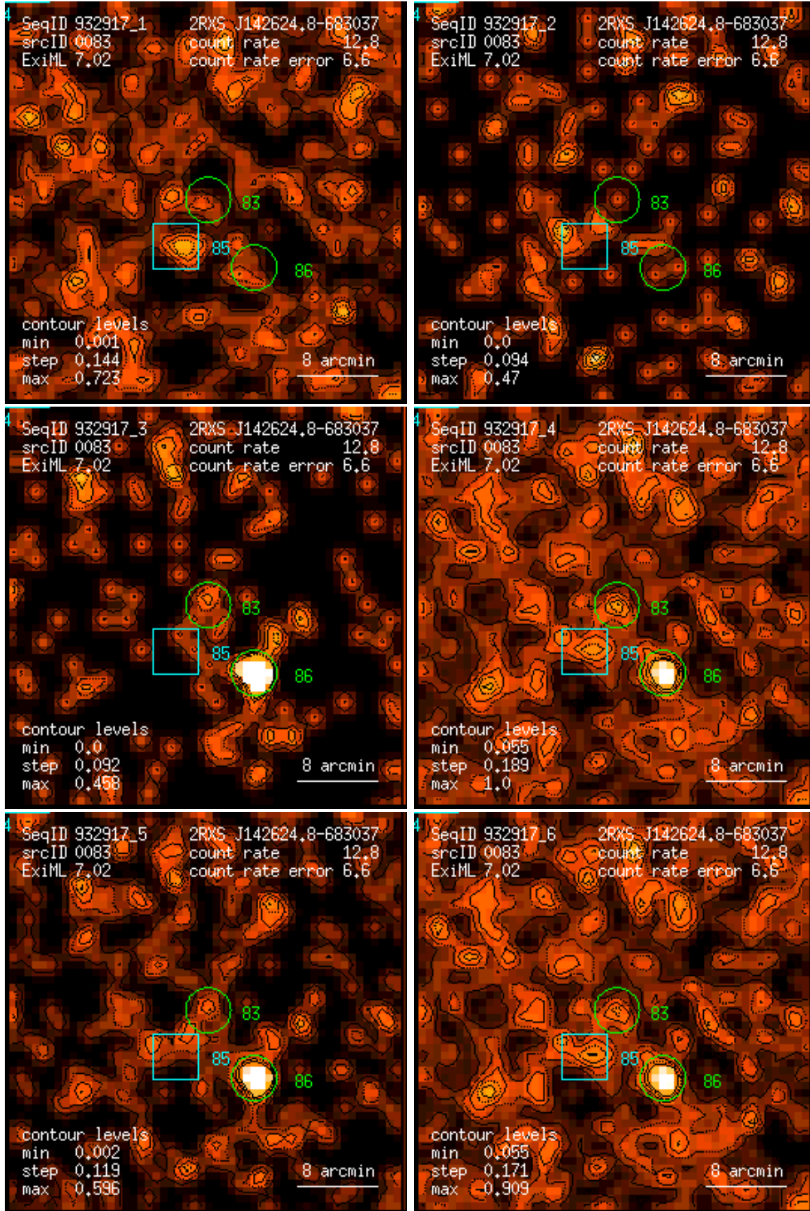
Figure 83: RASS 932917: detection 0083: band rate images, Gaussian filter: (1) PSPC channels 11 – 41, (2) 52 – 90, (3) 91 – 201, (4) 11 – 235, (5) 52 – 201, (6) 11 – 201. Broad band rates in counts/ks. Band rate contour levels in counts/ks/arcmin 2 .
