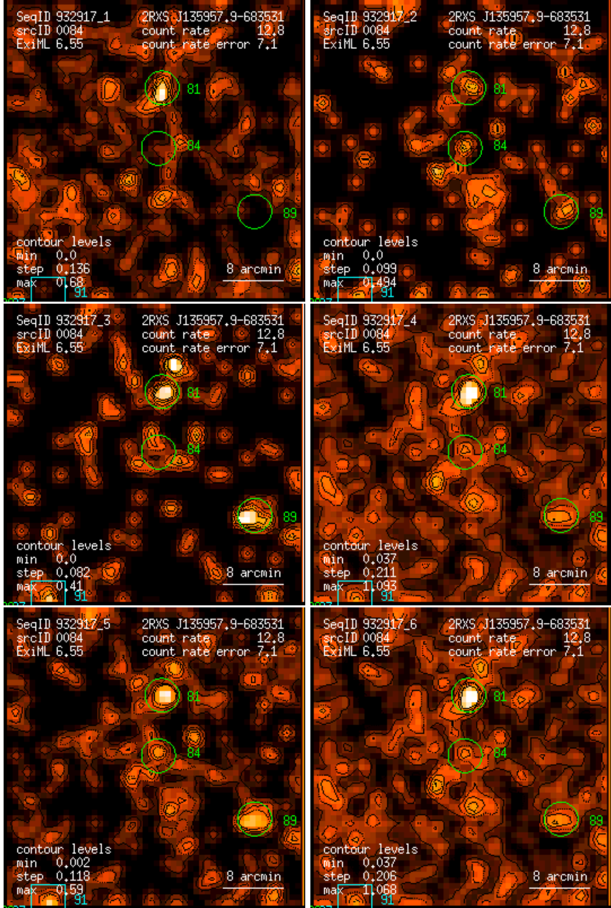
Figure 84: RASS 932917: detection 0084: band rate images, Gaussian filter: (1) PSPC channels 11 – 41, (2) 52 – 90, (3) 91 – 201, (4) 11 – 235, (5) 52 – 201, (6) 11 – 201. Broad band rates in counts/ks. Band rate contour levels in counts/ks/arcmin 2 .
