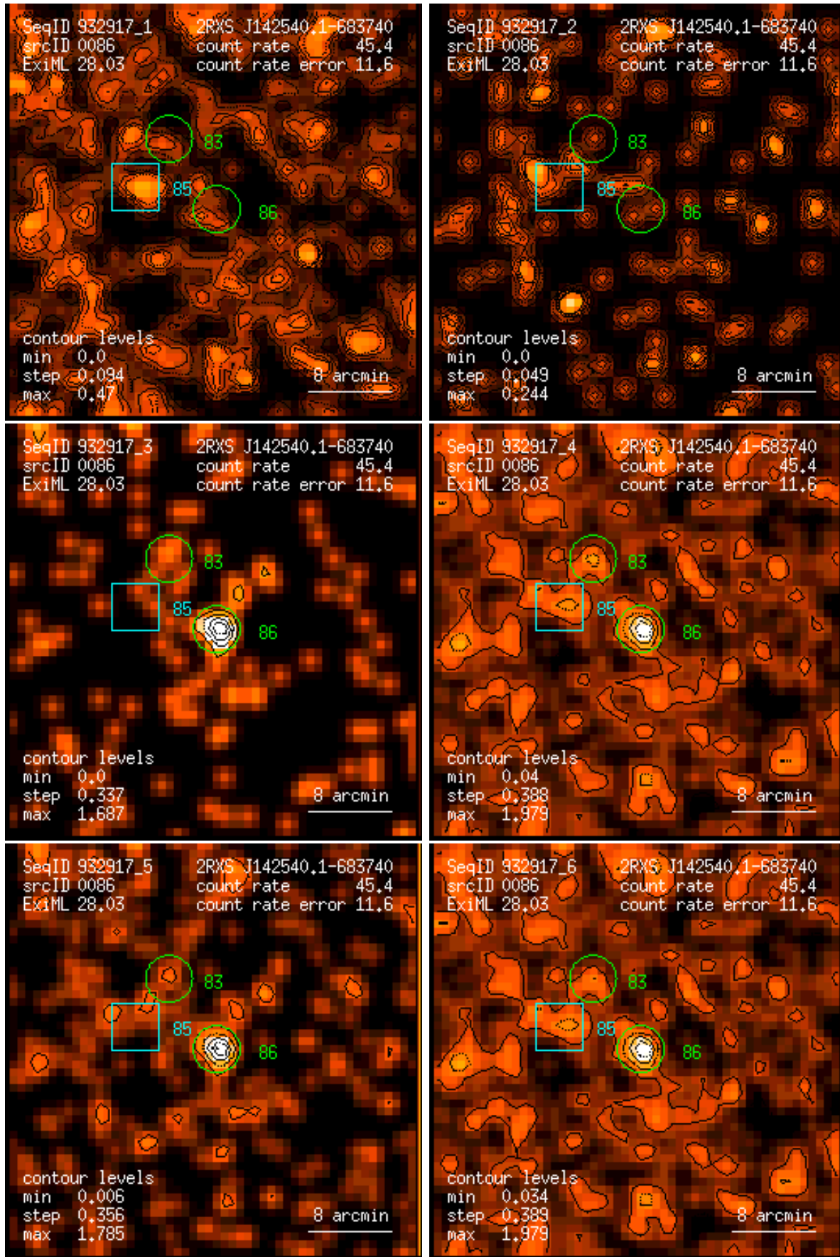
Figure 86: RASS 932917: detection 0086: band rate images, Gaussian filter: (1) PSPC channels 11 – 41, (2) 52 – 90, (3) 91 – 201, (4) 11 – 235, (5) 52 – 201, (6) 11 – 201. Broad band rates in counts/ks. Band rate contour levels in counts/ks/arcmin 2 .
