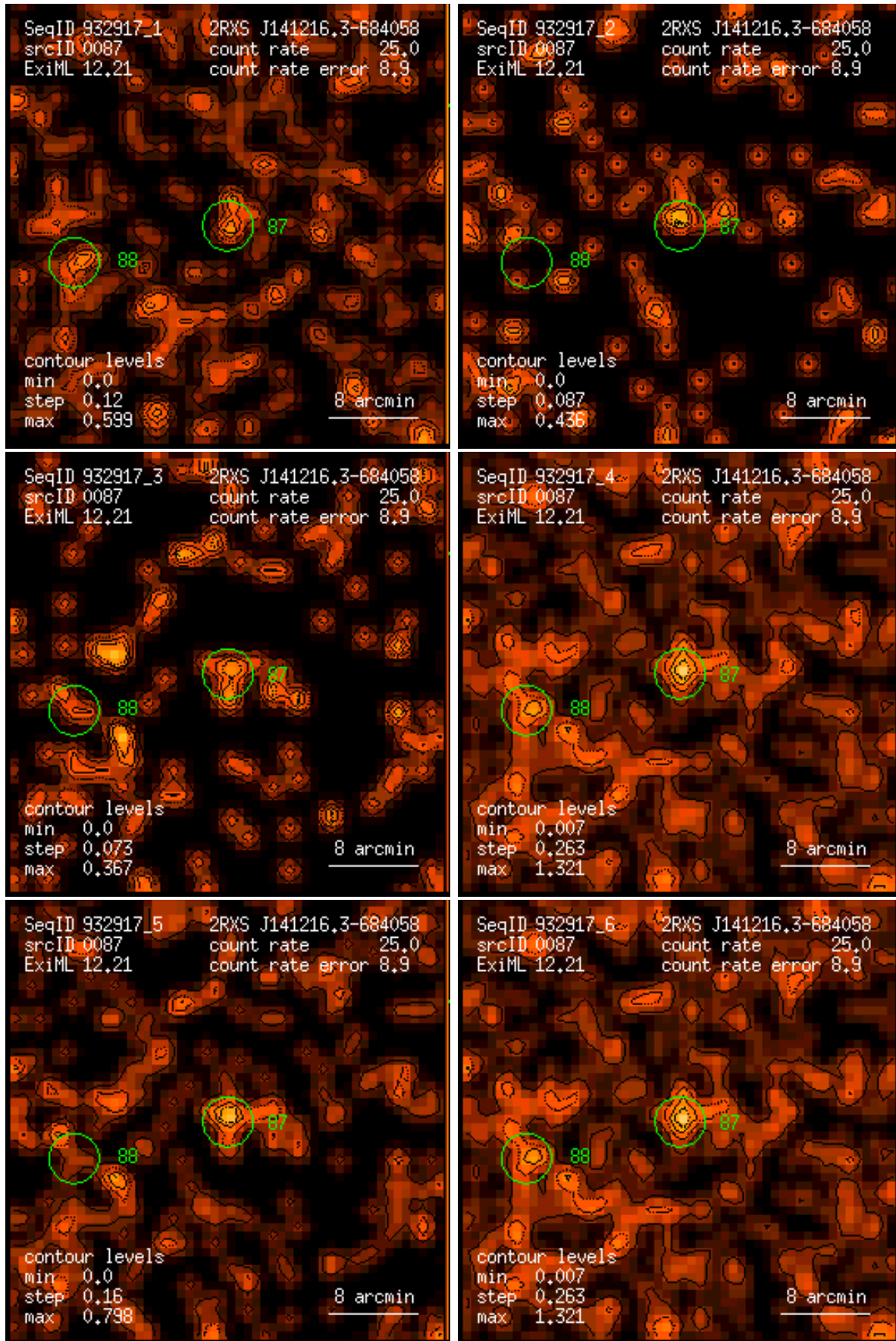
Figure 87: RASS 932917: detection 0087: band rate images, Gaussian filter: (1) PSPC channels 11 – 41, (2) 52 – 90, (3) 91 – 201, (4) 11 – 235, (5) 52 – 201, (6) 11 – 201. Broad band rates in counts/ks. Band rate contour levels in counts/ks/arcmin 2 .
