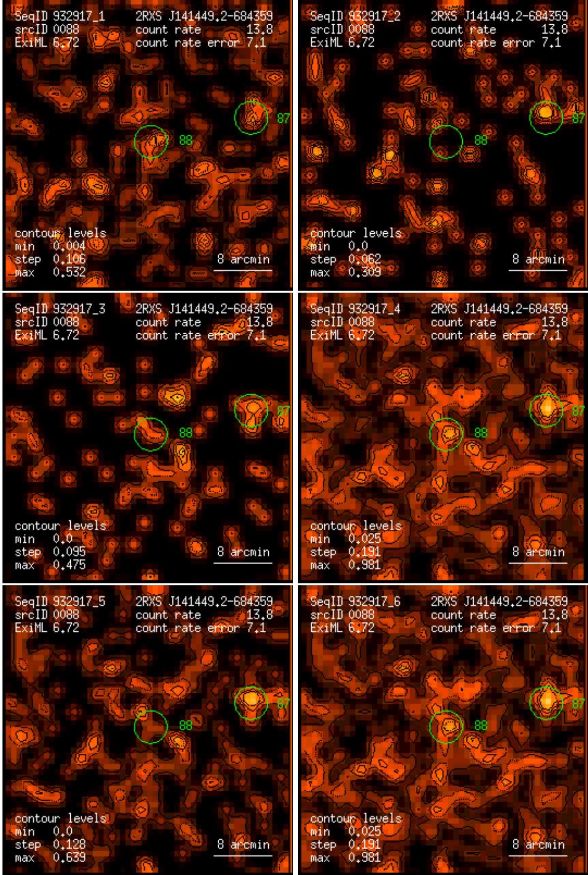
Figure 88: RASS 932917: detection 0088: band rate images, Gaussian filter: (1) PSPC channels 11 – 41, (2) 52 – 90, (3) 91 – 201, (4) 11 – 235, (5) 52 – 201, (6) 11 – 201. Broad band rates in counts/ks. Band rate contour levels in counts/ks/arcmin 2 .
