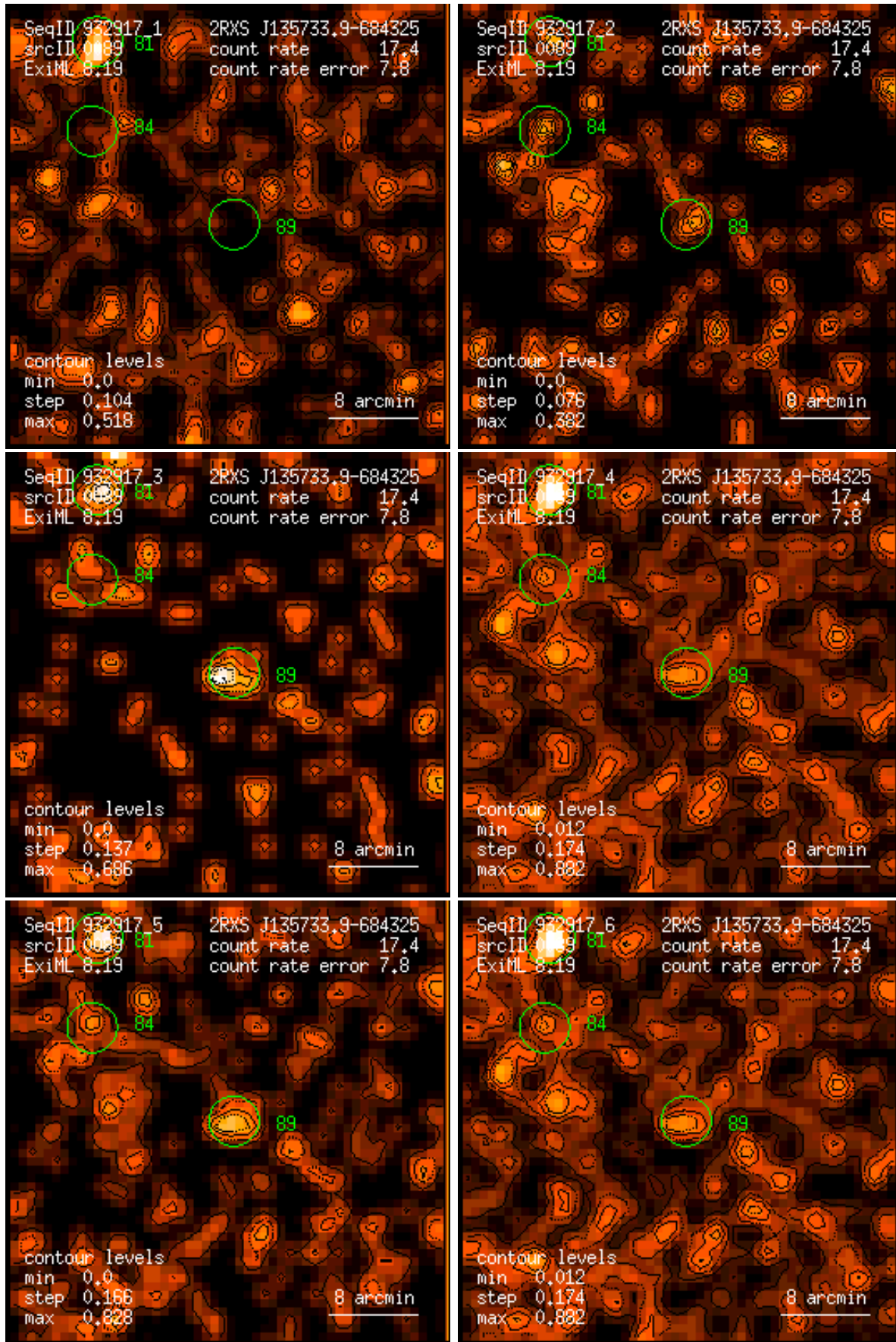
Figure 89: RASS 932917: detection 0089: band rate images, Gaussian filter: (1) PSPC channels 11 – 41, (2) 52 – 90, (3) 91 – 201, (4) 11 – 235, (5) 52 – 201, (6) 11 – 201. Broad band rates in counts/ks. Band rate contour levels in counts/ks/arcmin 2 .
