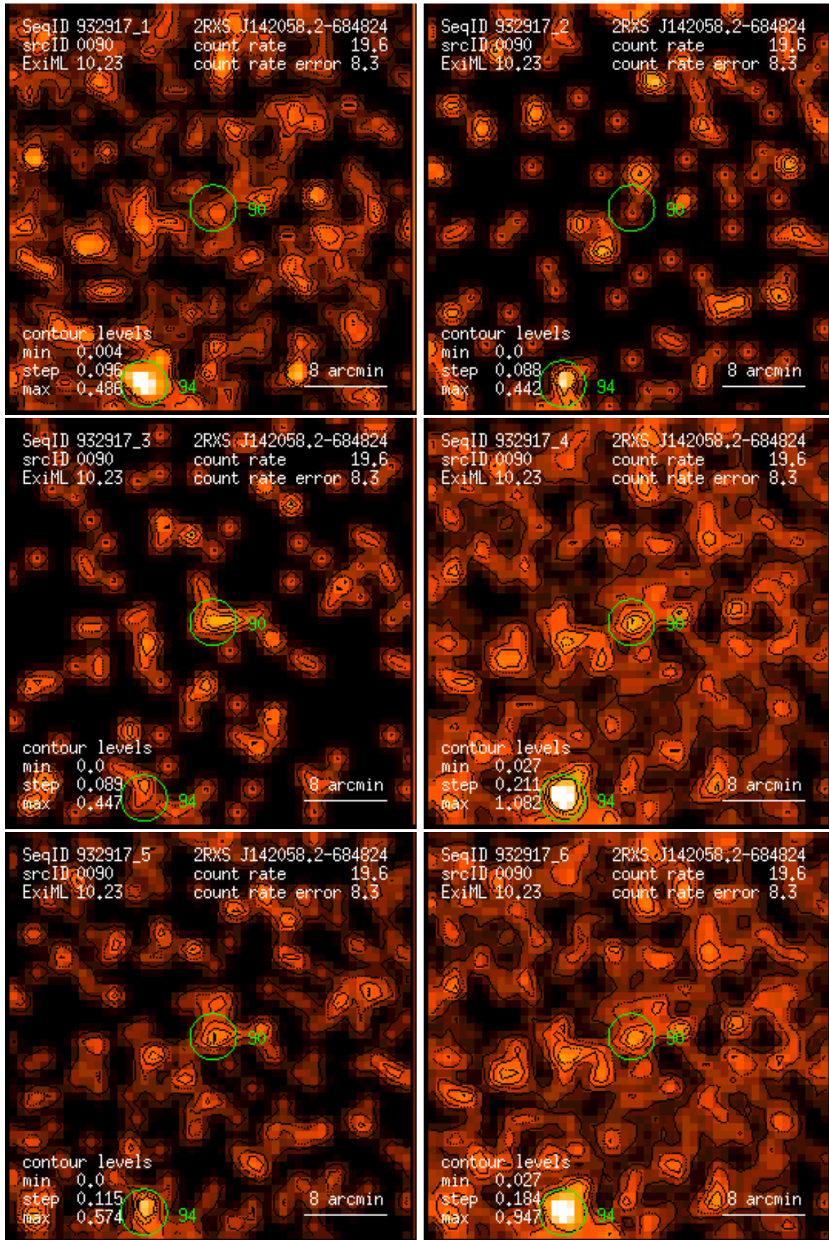
Figure 90: RASS 932917: detection 0090: band rate images, Gaussian filter: (1) PSPC channels 11 – 41, (2) 52 – 90, (3) 91 – 201, (4) 11 – 235, (5) 52 – 201, (6) 11 – 201. Broad band rates in counts/ks. Band rate contour levels in counts/ks/arcmin 2 .
