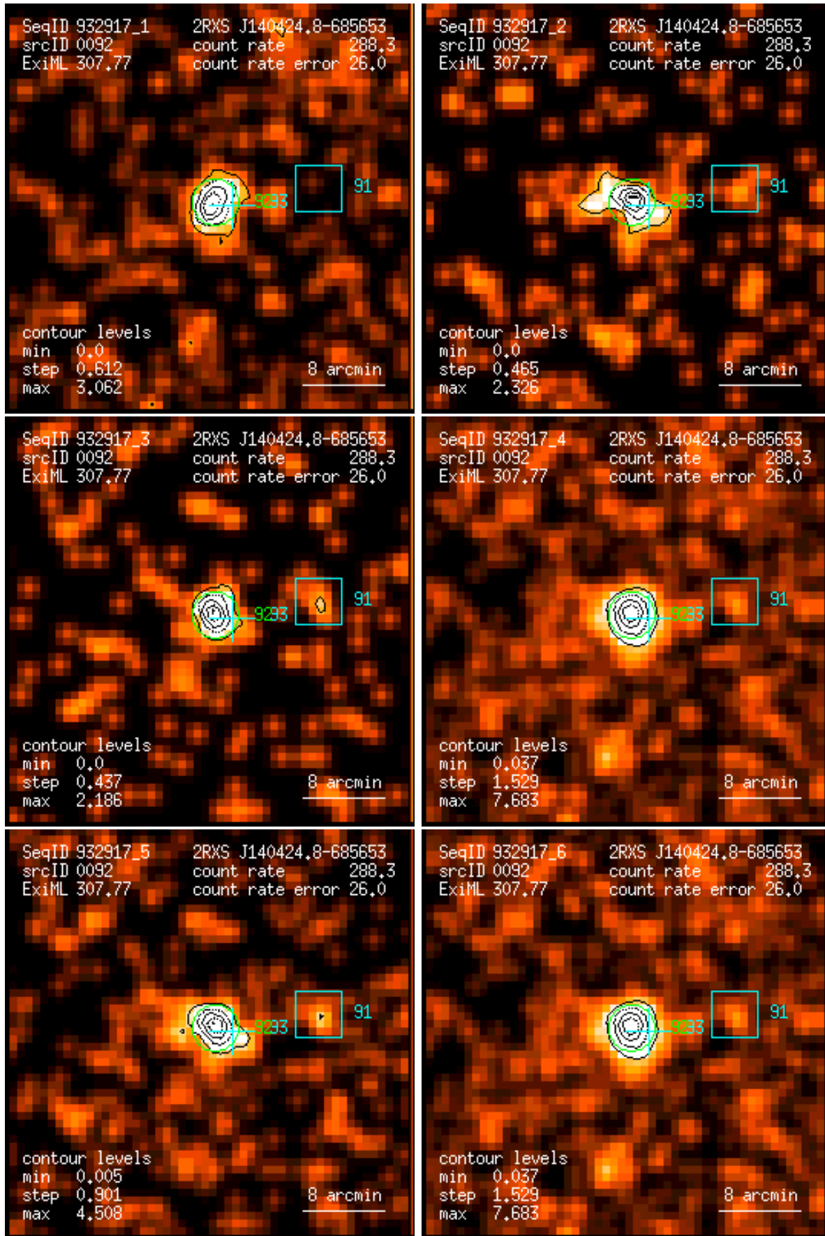
Figure 92: RASS 932917: detection 0092: band rate images, Gaussian filter: (1) PSPC channels 11 – 41, (2) 52 – 90, (3) 91 – 201, (4) 11 – 235, (5) 52 – 201, (6) 11 – 201. Broad band rates in counts/ks. Band rate contour levels in counts/ks/arcmin 2 .
