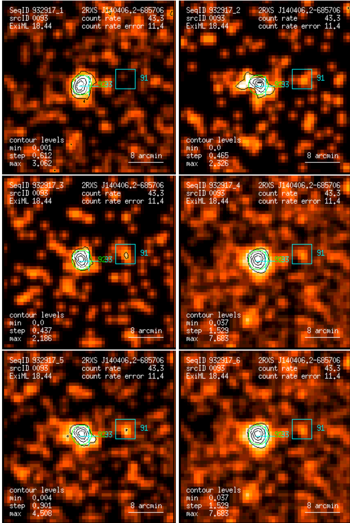
Figure 93: RASS 932917: detection 0093: band rate images, Gaussian filter: (1) PSPC channels 11 – 41, (2) 52 – 90, (3) 91 – 201, (4) 11 – 235, (5) 52 – 201, (6) 11 – 201. Broad band rates in counts/ks. Band rate contour levels in counts/ks/arcmin 2 .
