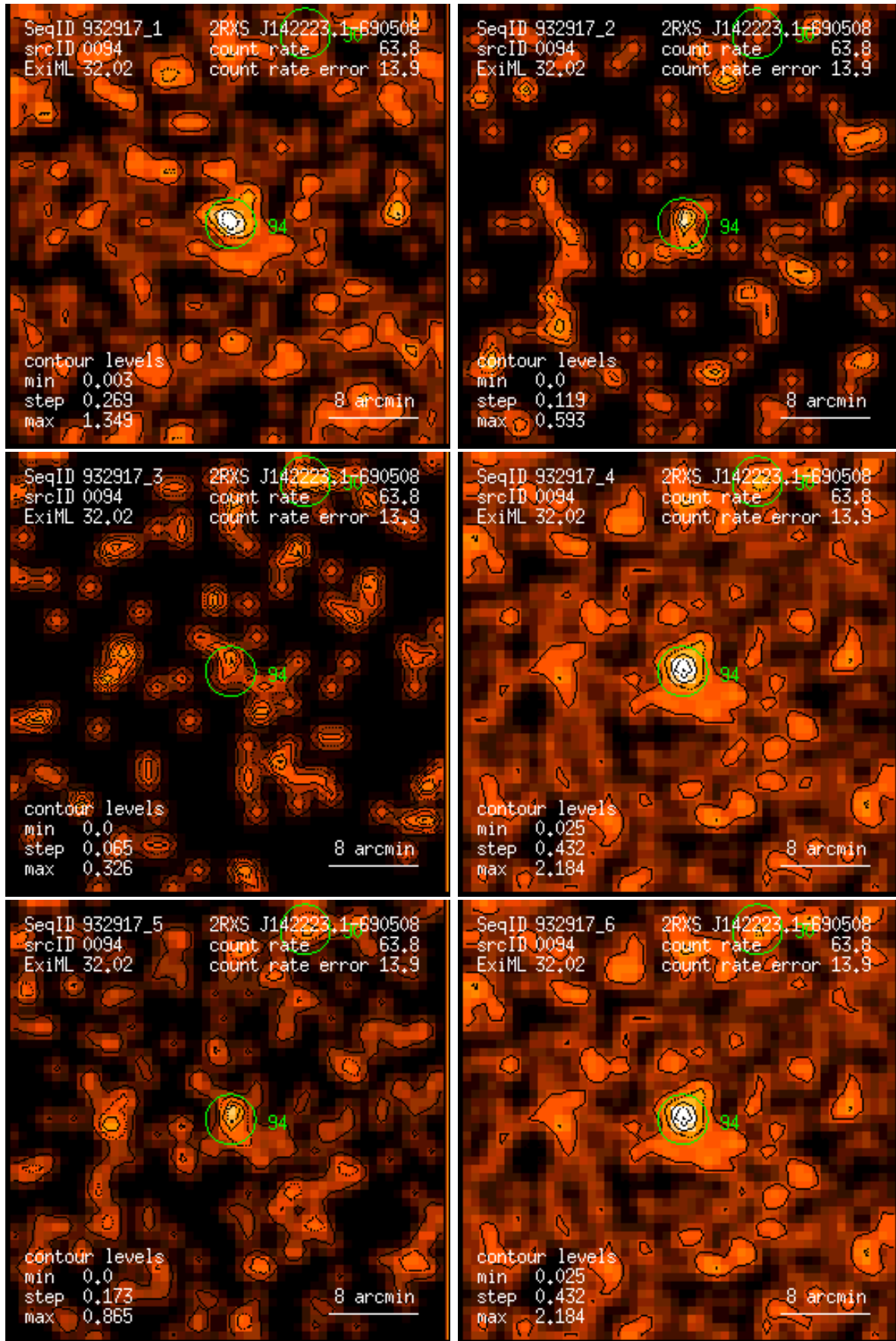
Figure 94: RASS 932917: detection 0094: band rate images, Gaussian filter: (1) PSPC channels 11 – 41, (2) 52 – 90, (3) 91 – 201, (4) 11 – 235, (5) 52 – 201, (6) 11 – 201. Broad band rates in counts/ks. Band rate contour levels in counts/ks/arcmin 2 .
