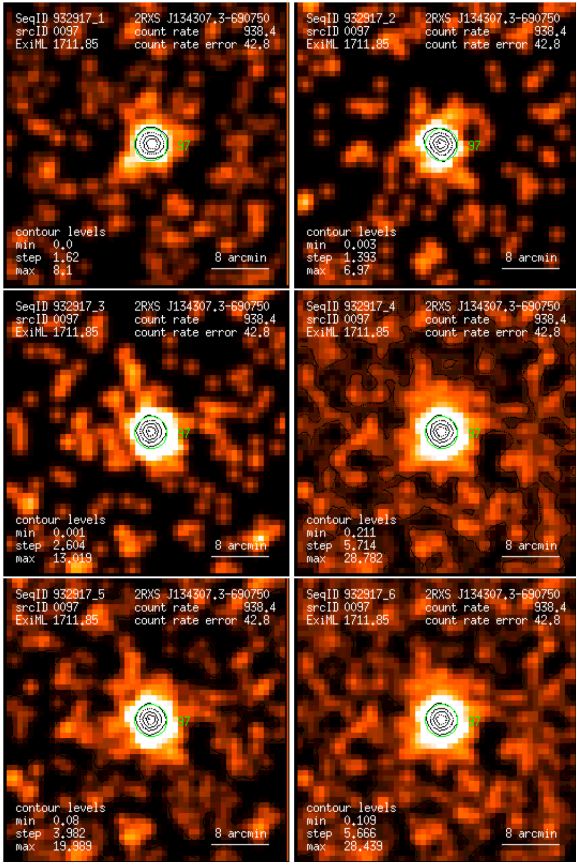
Figure 97: RASS 932917: detection 0097: band rate images, Gaussian filter: (1) PSPC channels 11 – 41, (2) 52 – 90, (3) 91 – 201, (4) 11 – 235, (5) 52 – 201, (6) 11 – 201. Broad band rates in counts/ks. Band rate contour levels in counts/ks/arcmin 2 .
