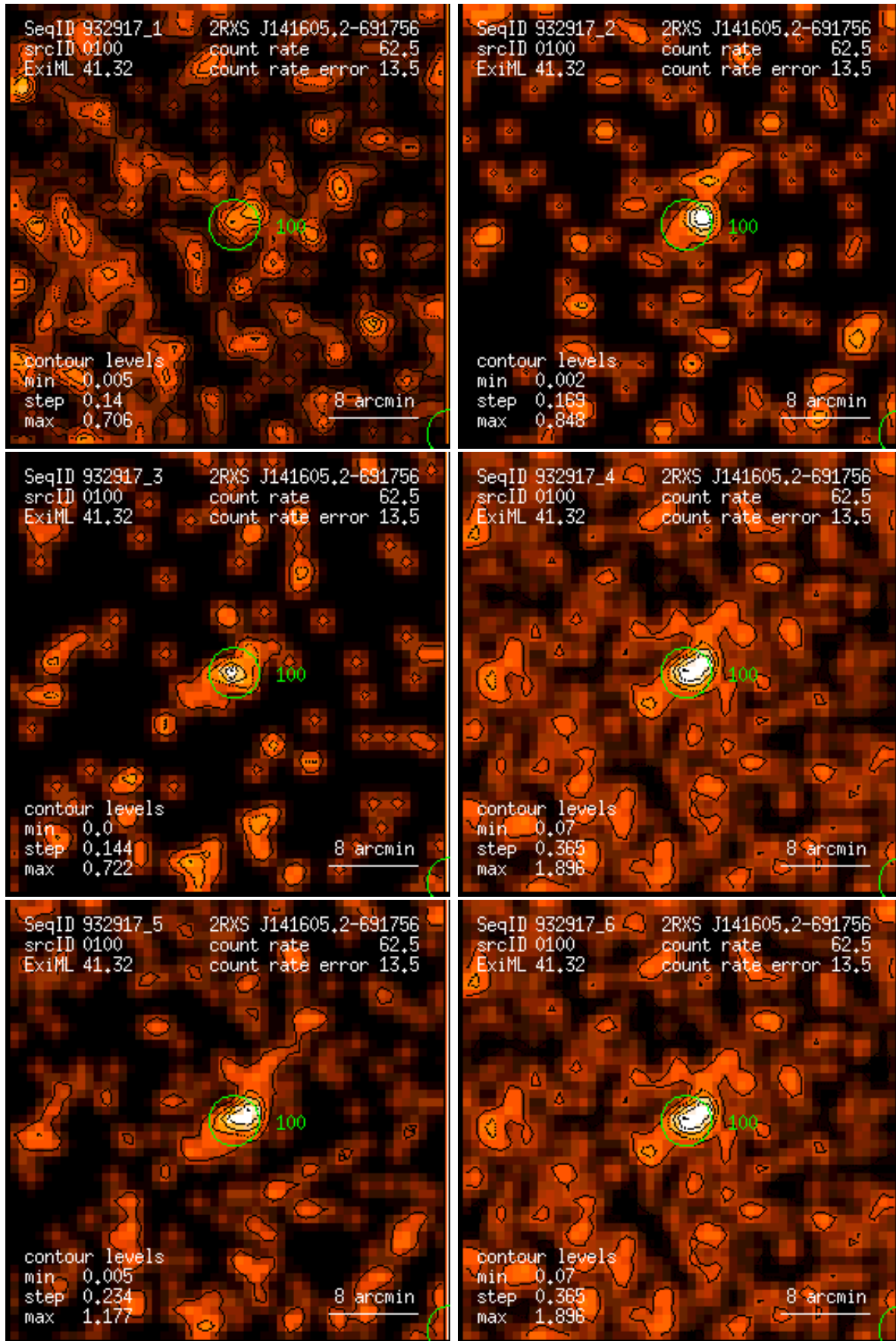
Figure 100: RASS 932917: detection 0100: band rate images, Gaussian filter: (1) PSPC channels 11 – 41, (2) 52 – 90, (3) 91 – 201, (4) 11 – 235, (5) 52 – 201, (6) 11 – 201. Broad band rates in counts/ks. Band rate contour levels in counts/ks/arcmin 2 .
