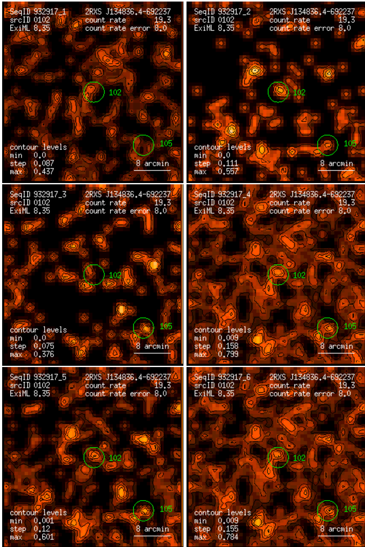
Figure 102: RASS 932917: detection 0102: band rate images, Gaussian filter: (1) PSPC channels 11 – 41, (2) 52 – 90, (3) 91 – 201, (4) 11 – 235, (5) 52 – 201, (6) 11 – 201. Broad band rates in counts/ks. Band rate contour levels in counts/ks/arcmin 2 .
