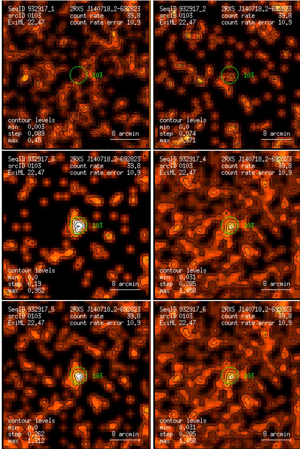
Figure 103: RASS 932917: detection 0103: band rate images, Gaussian filter: (1) PSPC channels 11 – 41, (2) 52 – 90, (3) 91 – 201, (4) 11 – 235, (5) 52 – 201, (6) 11 – 201. Broad band rates in counts/ks. Band rate contour levels in counts/ks/arcmin 2 .
