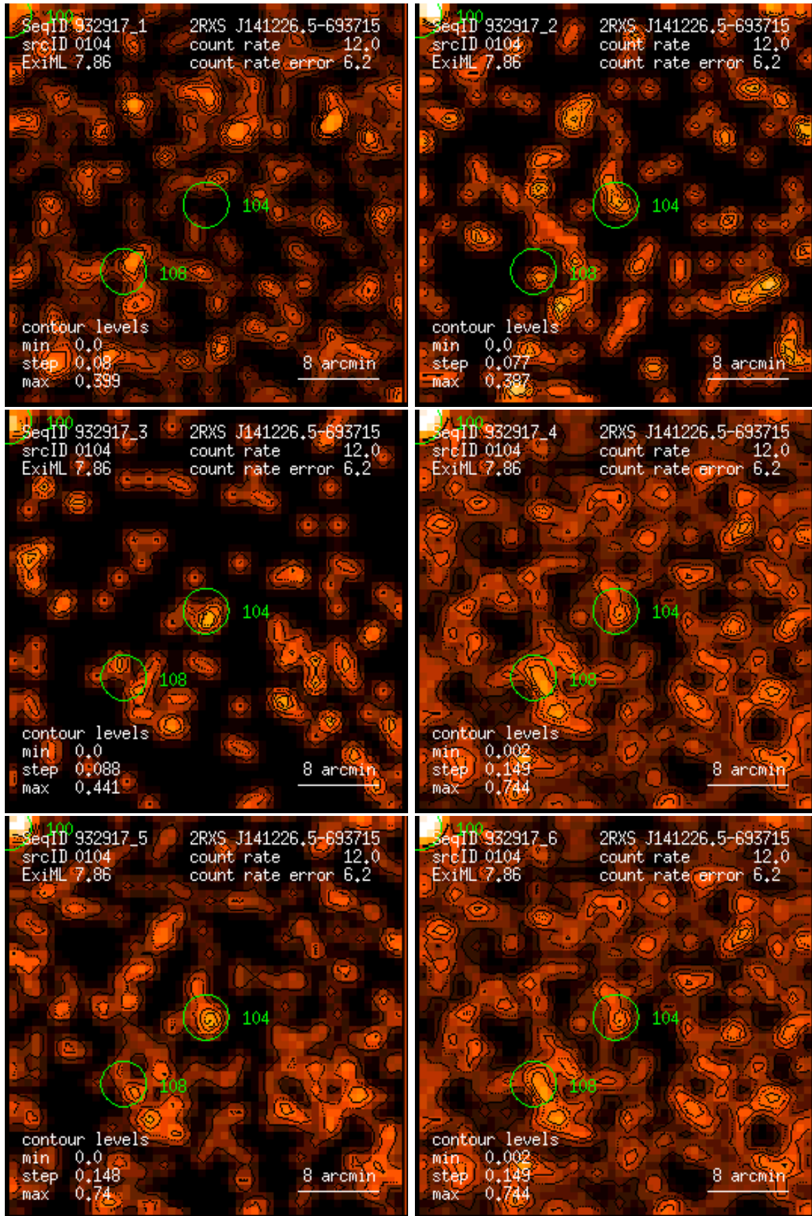
Figure 104: RASS 932917: detection 0104: band rate images, Gaussian filter: (1) PSPC channels 11 – 41, (2) 52 – 90, (3) 91 – 201, (4) 11 – 235, (5) 52 – 201, (6) 11 – 201. Broad band rates in counts/ks. Band rate contour levels in counts/ks/arcmin 2 .
