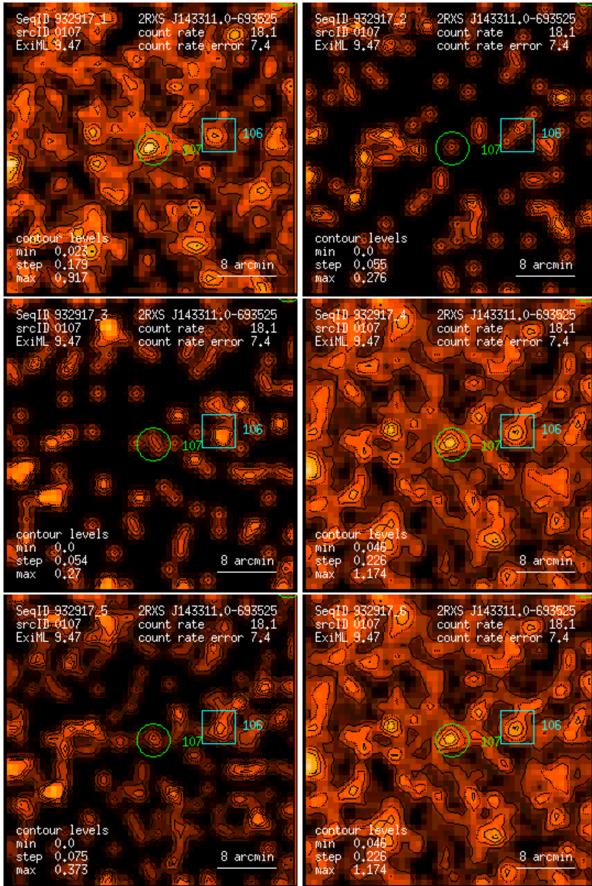
Figure 107: RASS 932917: detection 0107: band rate images, Gaussian filter: (1) PSPC channels 11 – 41, (2) 52 – 90, (3) 91 – 201, (4) 11 – 235, (5) 52 – 201, (6) 11 – 201. Broad band rates in counts/ks. Band rate contour levels in counts/ks/arcmin 2 .
