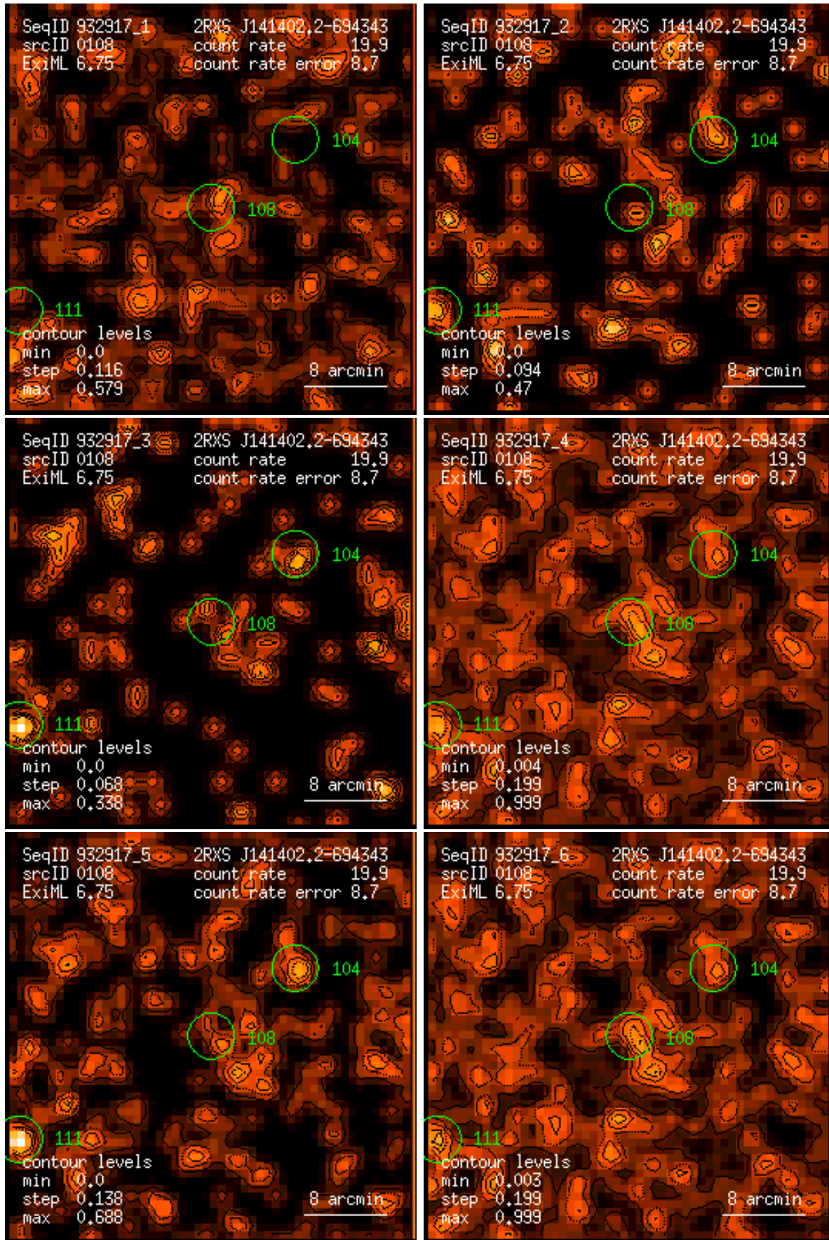
Figure 108: RASS 932917: detection 0108: band rate images, Gaussian filter: (1) PSPC channels 11 – 41, (2) 52 – 90, (3) 91 – 201, (4) 11 – 235, (5) 52 – 201, (6) 11 – 201. Broad band rates in counts/ks. Band rate contour levels in counts/ks/arcmin 2 .
