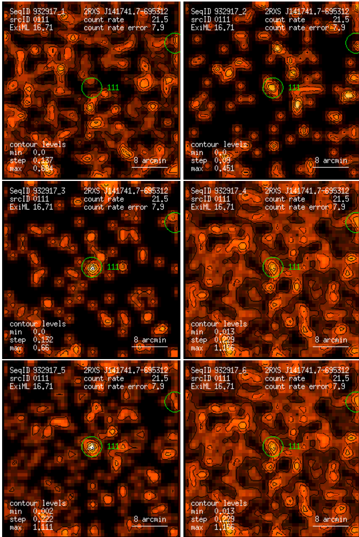
Figure 111: RASS 932917: detection 0111: band rate images, Gaussian filter: (1) PSPC channels 11 – 41, (2) 52 – 90, (3) 91 – 201, (4) 11 – 235, (5) 52 – 201, (6) 11 – 201. Broad band rates in counts/ks. Band rate contour levels in counts/ks/arcmin 2 .
