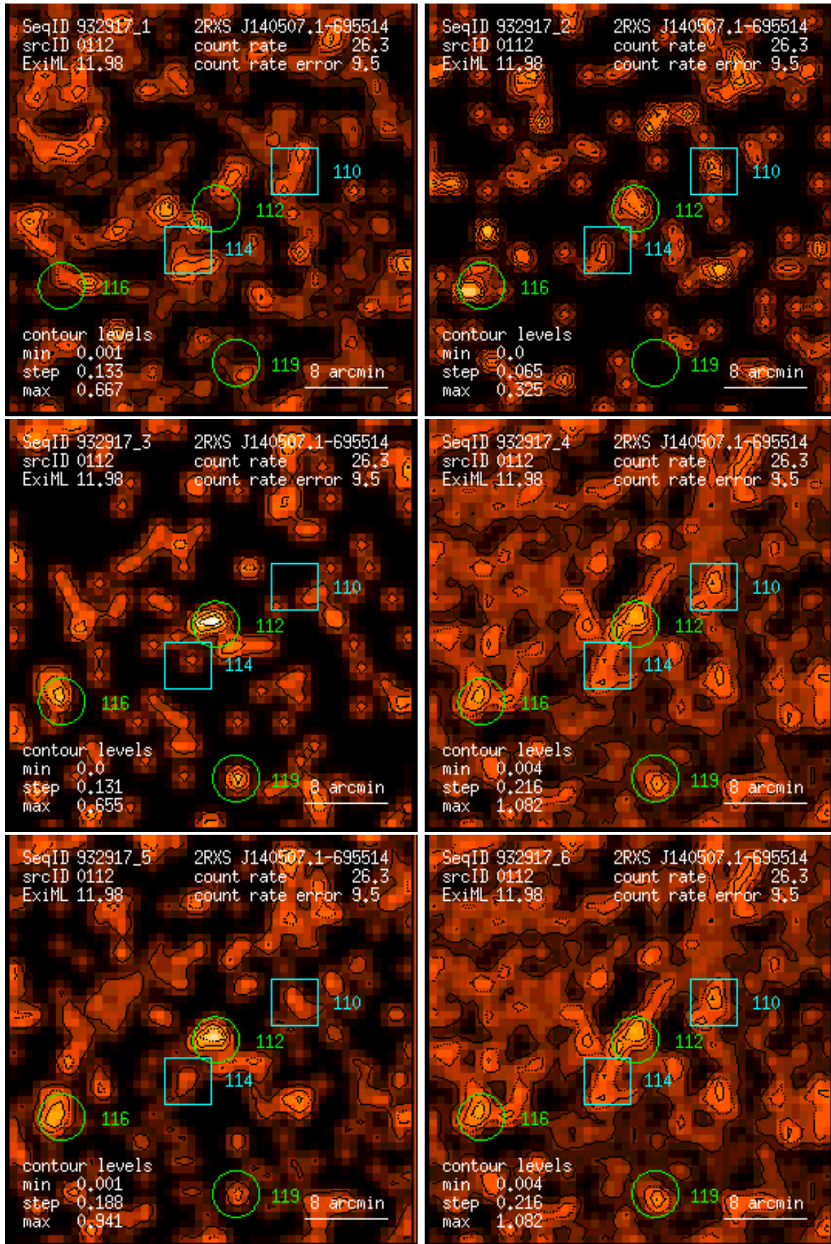
Figure 112: RASS 932917: detection 0112: band rate images, Gaussian filter: (1) PSPC channels 11 – 41, (2) 52 – 90, (3) 91 – 201, (4) 11 – 235, (5) 52 – 201, (6) 11 – 201. Broad band rates in counts/ks. Band rate contour levels in counts/ks/arcmin 2 .
