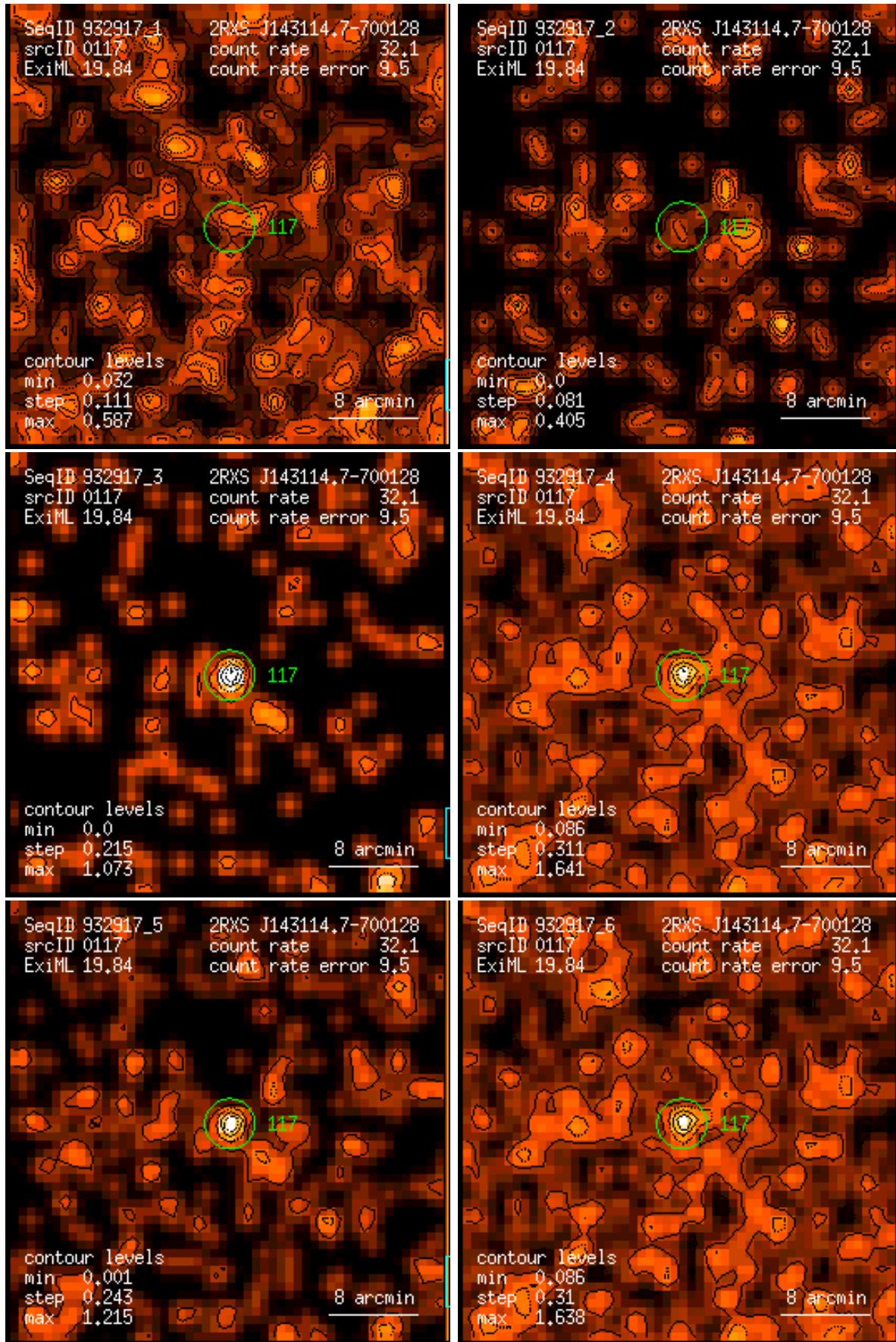
Figure 117: RASS 932917: detection 0117: band rate images, Gaussian filter: (1) PSPC channels 11 – 41, (2) 52 – 90, (3) 91 – 201, (4) 11 – 235, (5) 52 – 201, (6) 11 – 201. Broad band rates in counts/ks. Band rate contour levels in counts/ks/arcmin 2 .
