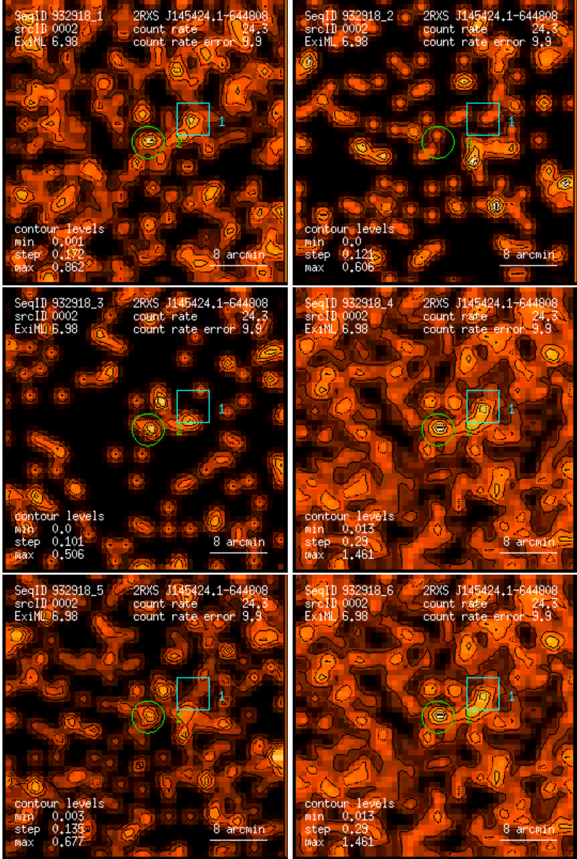
Figure 2: RASS 932918: detection 0002: band rate images, Gaussian filter: (1) PSPC channels 11 – 41, (2) 52 – 90, (3) 91 – 201, (4) 11 – 235, (5) 52 – 201, (6) 11 – 201. Broad band rates in counts/ks. Band rate contour levels in counts/ks/arcmin 2 .
