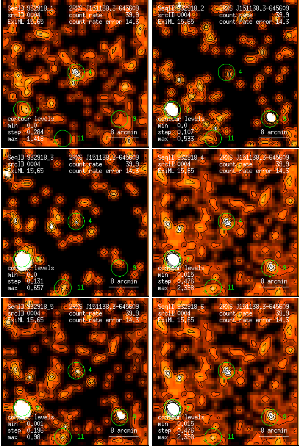
Figure 4: RASS 932918: detection 0004: band rate images, Gaussian filter: (1) PSPC channels 11 – 41, (2) 52 – 90, (3) 91 – 201, (4) 11 – 235, (5) 52 – 201, (6) 11 – 201. Broad band rates in counts/ks. Band rate contour levels in counts/ks/arcmin 2 .
