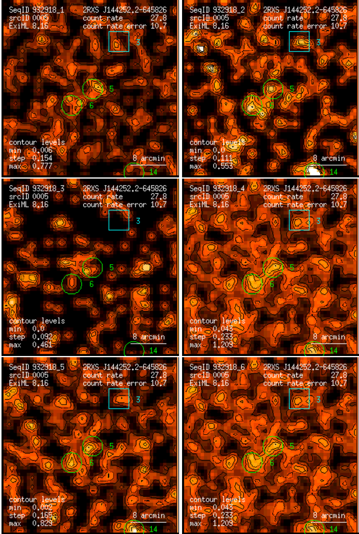
Figure 5: RASS 932918: detection 0005: band rate images, Gaussian filter: (1) PSPC channels 11 – 41, (2) 52 – 90, (3) 91 – 201, (4) 11 – 235, (5) 52 – 201, (6) 11 – 201. Broad band rates in counts/ks. Band rate contour levels in counts/ks/arcmin 2 .
