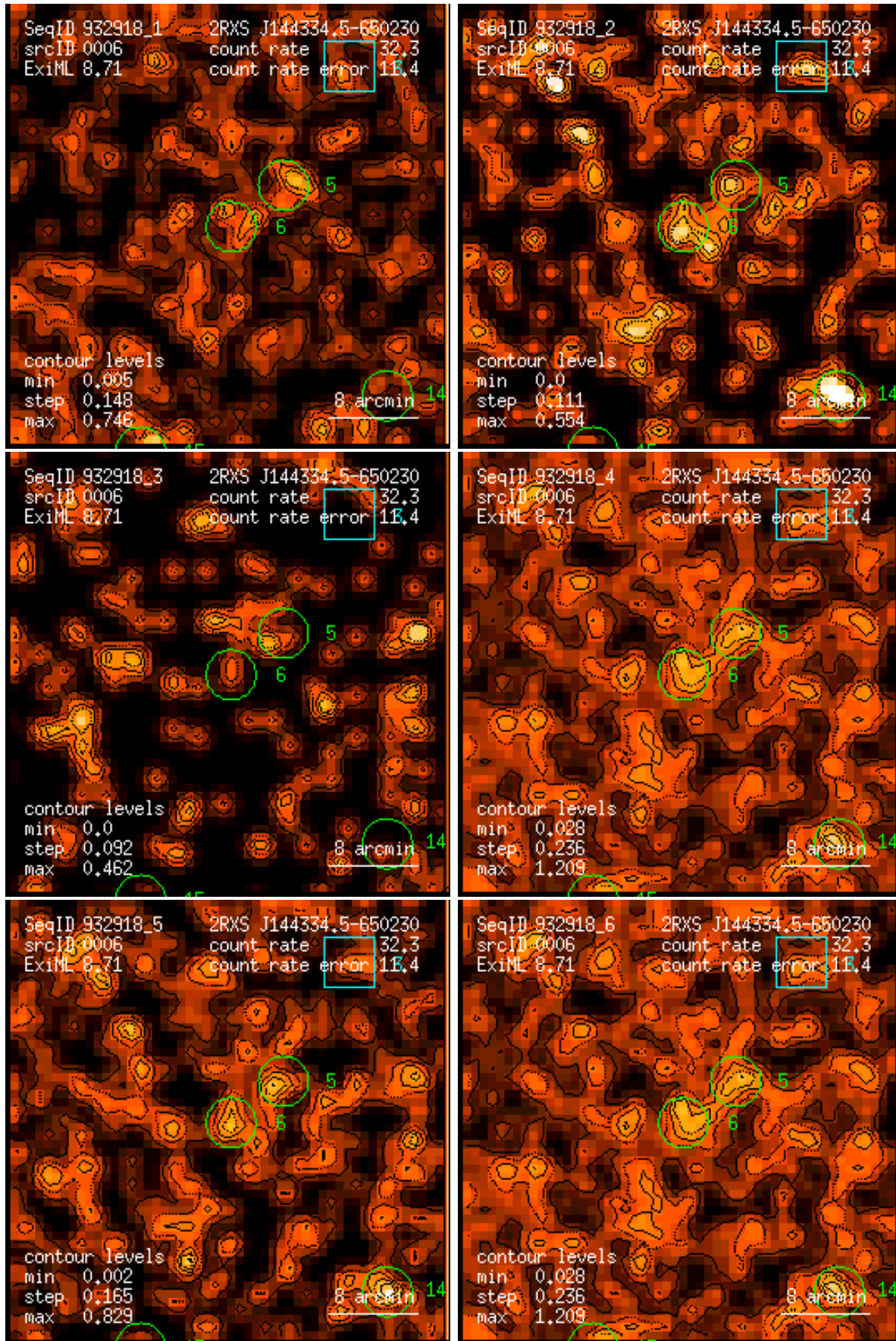
Figure 6: RASS 932918: detection 0006: band rate images, Gaussian filter: (1) PSPC channels 11 – 41, (2) 52 – 90, (3) 91 – 201, (4) 11 – 235, (5) 52 – 201, (6) 11 – 201. Broad band rates in counts/ks. Band rate contour levels in counts/ks/arcmin 2 .
