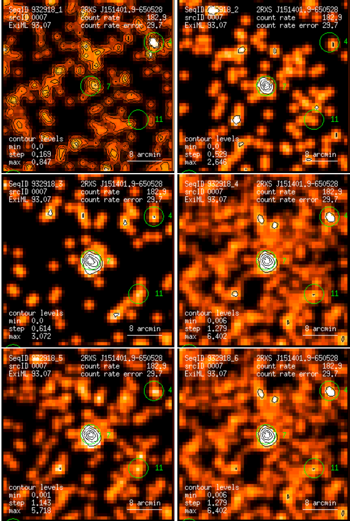
Figure 7: RASS 932918: detection 0007: band rate images, Gaussian filter: (1) PSPC channels 11 – 41, (2) 52 – 90, (3) 91 – 201, (4) 11 – 235, (5) 52 – 201, (6) 11 – 201. Broad band rates in counts/ks. Band rate contour levels in counts/ks/arcmin 2 .
