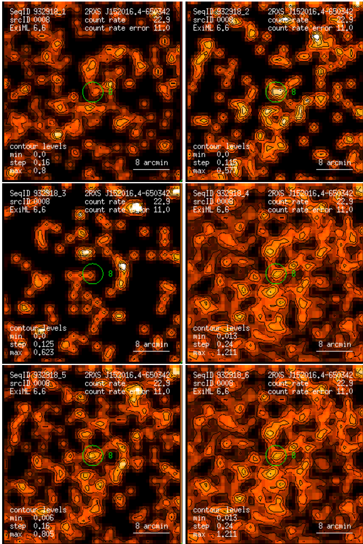
Figure 8: RASS 932918: detection 0008: band rate images, Gaussian filter: (1) PSPC channels 11 – 41, (2) 52 – 90, (3) 91 – 201, (4) 11 – 235, (5) 52 – 201, (6) 11 – 201. Broad band rates in counts/ks. Band rate contour levels in counts/ks/arcmin 2 .
