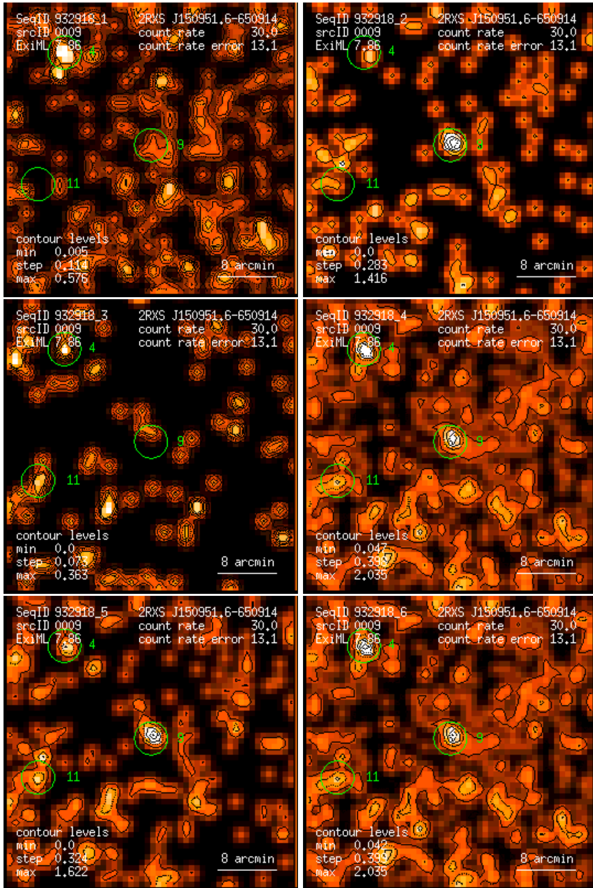
Figure 9: RASS 932918: detection 0009: band rate images, Gaussian filter: (1) PSPC channels 11 – 41, (2) 52 – 90, (3) 91 – 201, (4) 11 – 235, (5) 52 – 201, (6) 11 – 201. Broad band rates in counts/ks. Band rate contour levels in counts/ks/arcmin 2 .
