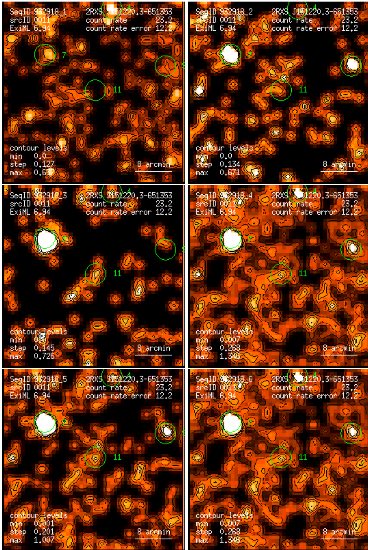
Figure 11: RASS 932918: detection 0011: band rate images, Gaussian filter: (1) PSPC channels 11 – 41, (2) 52 – 90, (3) 91 – 201, (4) 11 – 235, (5) 52 – 201, (6) 11 – 201. Broad band rates in counts/ks. Band rate contour levels in counts/ks/arcmin 2 .
