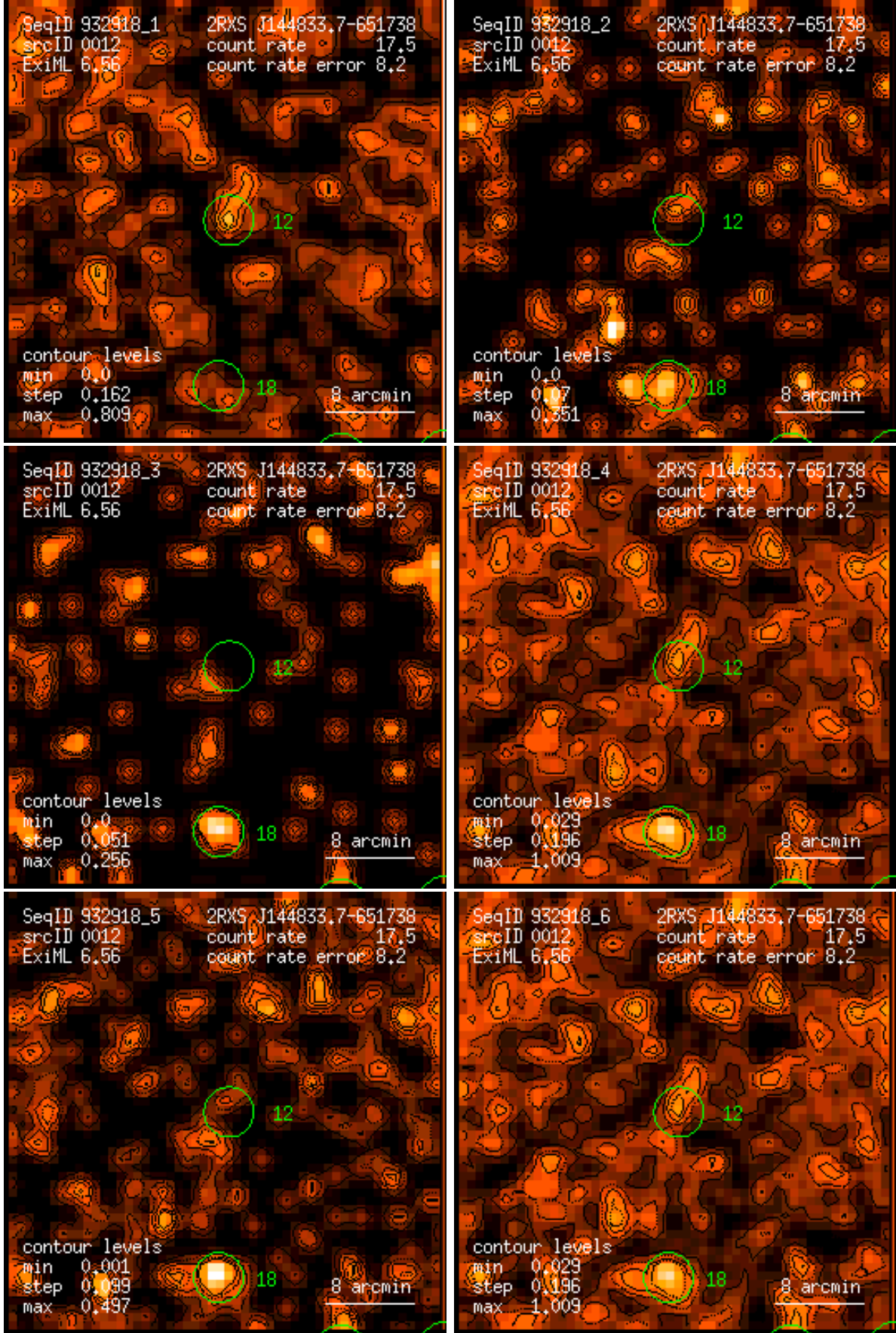
Figure 12: RASS 932918: detection 0012: band rate images, Gaussian filter: (1) PSPC channels 11 – 41, (2) 52 – 90, (3) 91 – 201, (4) 11 – 235, (5) 52 – 201, (6) 11 – 201. Broad band rates in counts/ks. Band rate contour levels in counts/ks/arcmin 2 .
