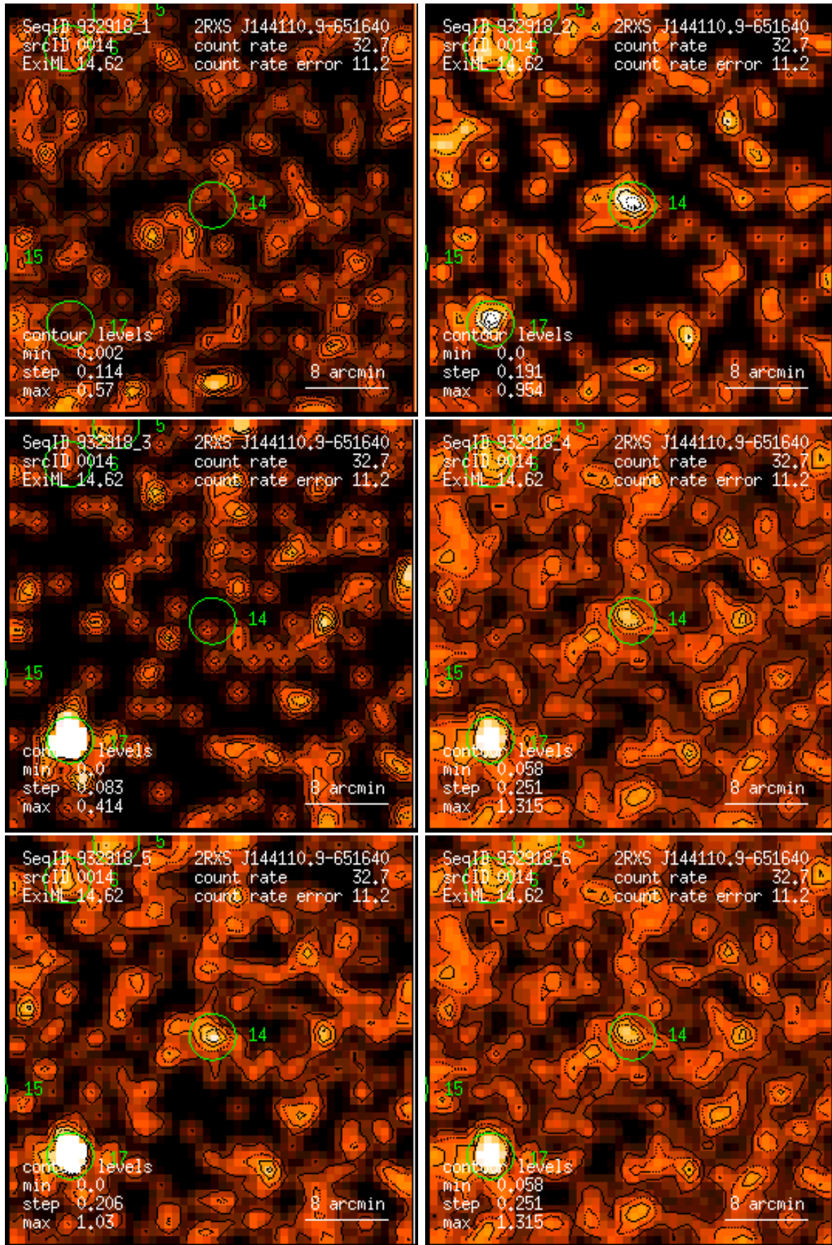
Figure 14: RASS 932918: detection 0014: band rate images, Gaussian filter: (1) PSPC channels 11 – 41, (2) 52 – 90, (3) 91 – 201, (4) 11 – 235, (5) 52 – 201, (6) 11 – 201. Broad band rates in counts/ks. Band rate contour levels in counts/ks/arcmin 2 .
