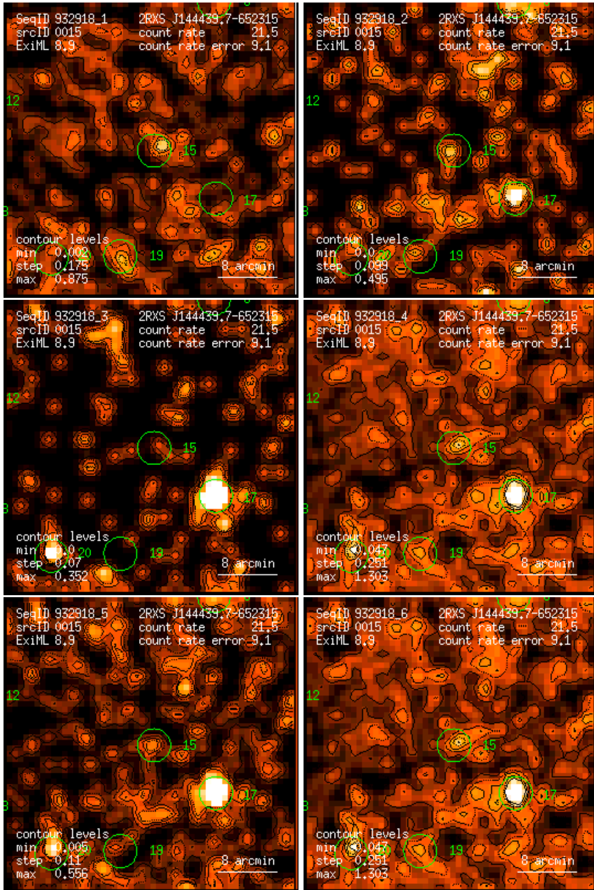
Figure 15: RASS 932918: detection 0015: band rate images, Gaussian filter: (1) PSPC channels 11 – 41, (2) 52 – 90, (3) 91 – 201, (4) 11 – 235, (5) 52 – 201, (6) 11 – 201. Broad band rates in counts/ks. Band rate contour levels in counts/ks/arcmin 2 .
