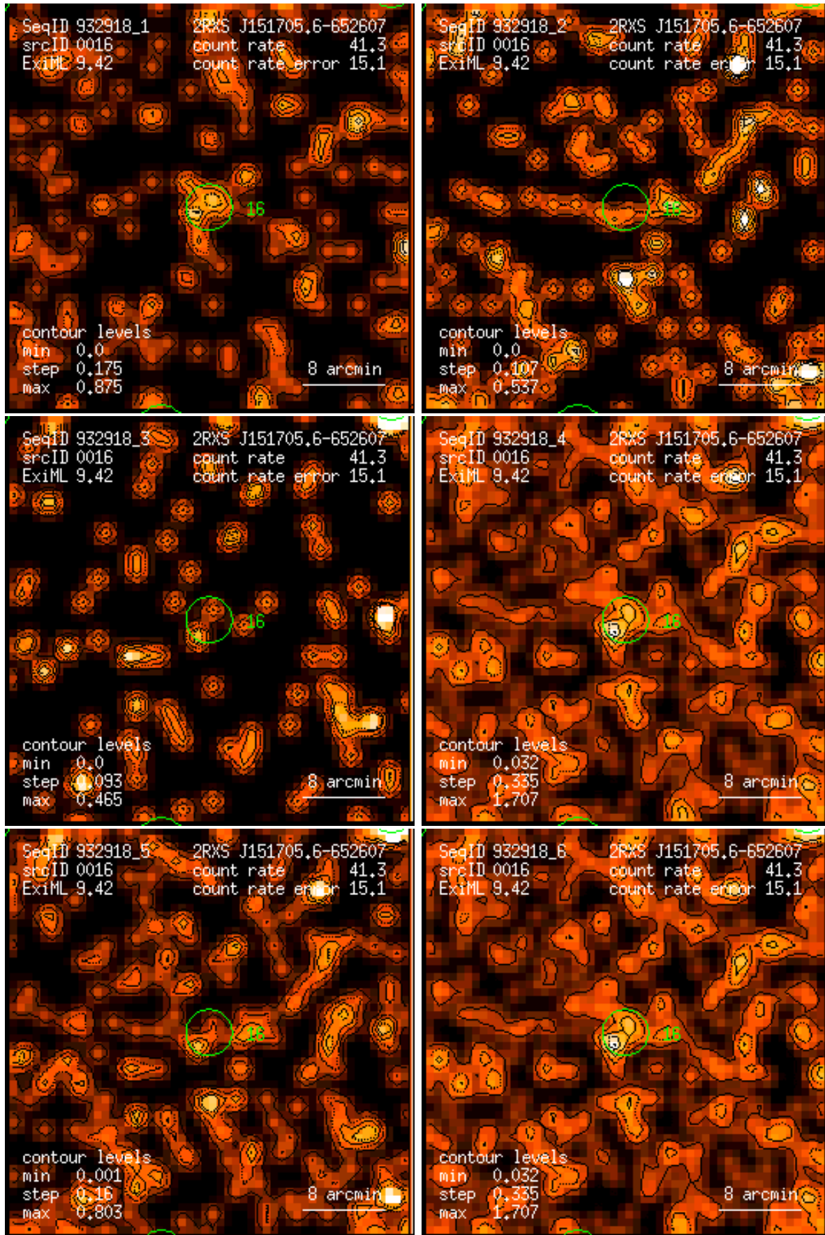
Figure 16: RASS 932918: detection 0016: band rate images, Gaussian filter: (1) PSPC channels 11 – 41, (2) 52 – 90, (3) 91 – 201, (4) 11 – 235, (5) 52 – 201, (6) 11 – 201. Broad band rates in counts/ks. Band rate contour levels in counts/ks/arcmin 2 .
