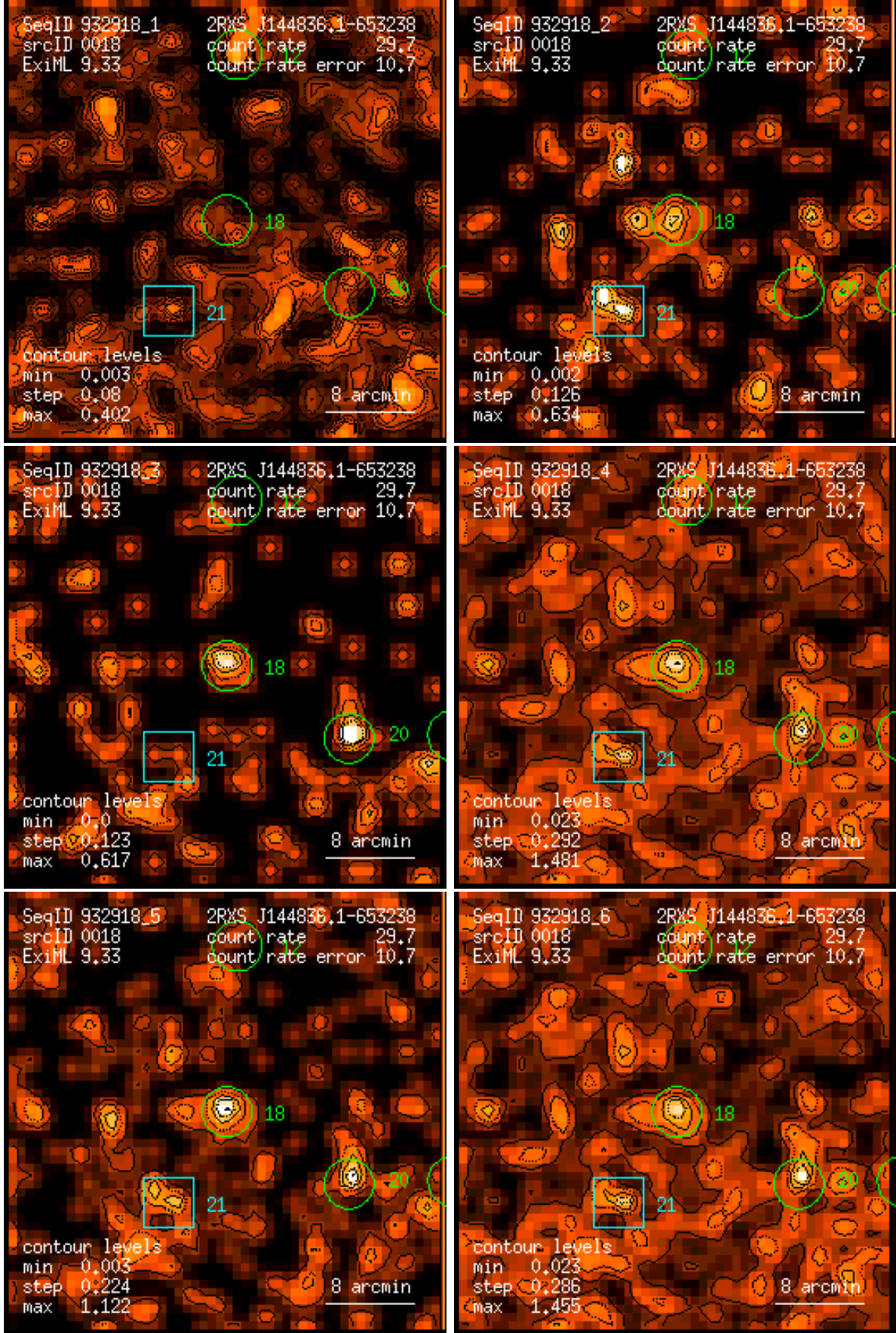
Figure 18: RASS 932918: detection 0018: band rate images, Gaussian filter: (1) PSPC channels 11 – 41, (2) 52 – 90, (3) 91 – 201, (4) 11 – 235, (5) 52 – 201, (6) 11 – 201. Broad band rates in counts/ks. Band rate contour levels in counts/ks/arcmin 2 .
