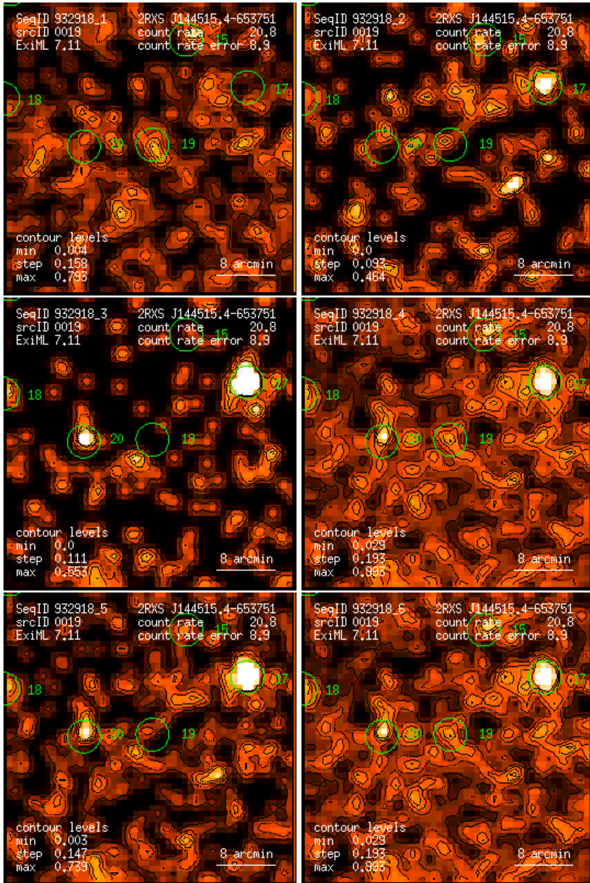
Figure 19: RASS 932918: detection 0019: band rate images, Gaussian filter: (1) PSPC channels 11 – 41, (2) 52 – 90, (3) 91 – 201, (4) 11 – 235, (5) 52 – 201, (6) 11 – 201. Broad band rates in counts/ks. Band rate contour levels in counts/ks/arcmin 2 .
