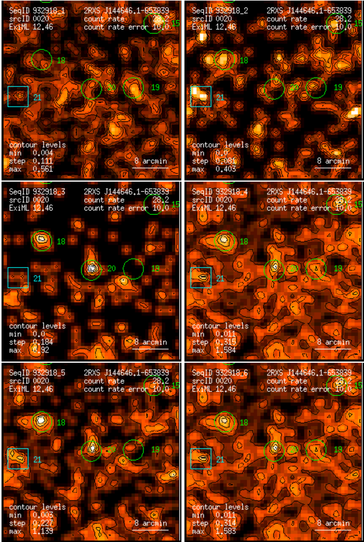
Figure 20: RASS 932918: detection 0020: band rate images, Gaussian filter: (1) PSPC channels 11 – 41, (2) 52 – 90, (3) 91 – 201, (4) 11 – 235, (5) 52 – 201, (6) 11 – 201. Broad band rates in counts/ks. Band rate contour levels in counts/ks/arcmin 2 .
