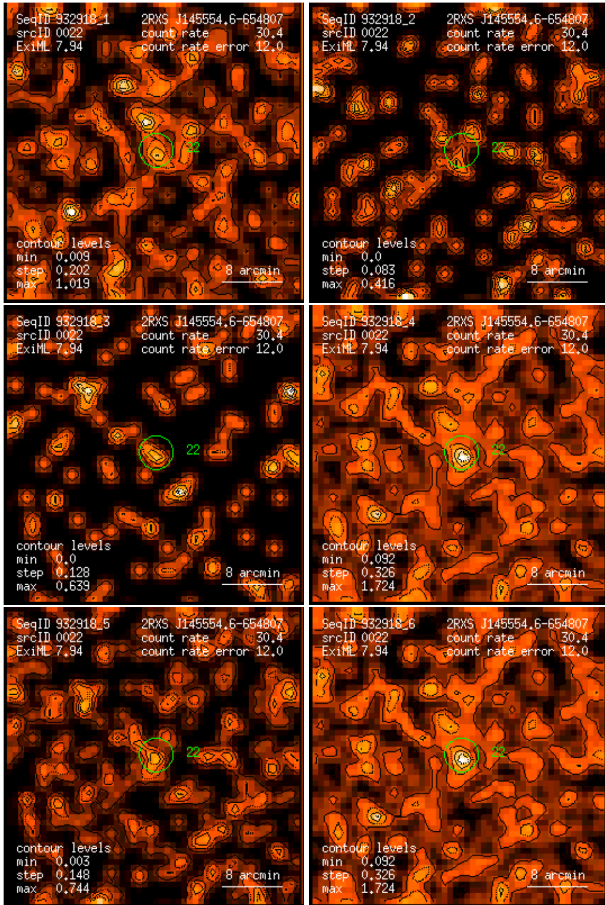
Figure 22: RASS 932918: detection 0022: band rate images, Gaussian filter: (1) PSPC channels 11 – 41, (2) 52 – 90, (3) 91 – 201, (4) 11 – 235, (5) 52 – 201, (6) 11 – 201. Broad band rates in counts/ks. Band rate contour levels in counts/ks/arcmin 2 .
