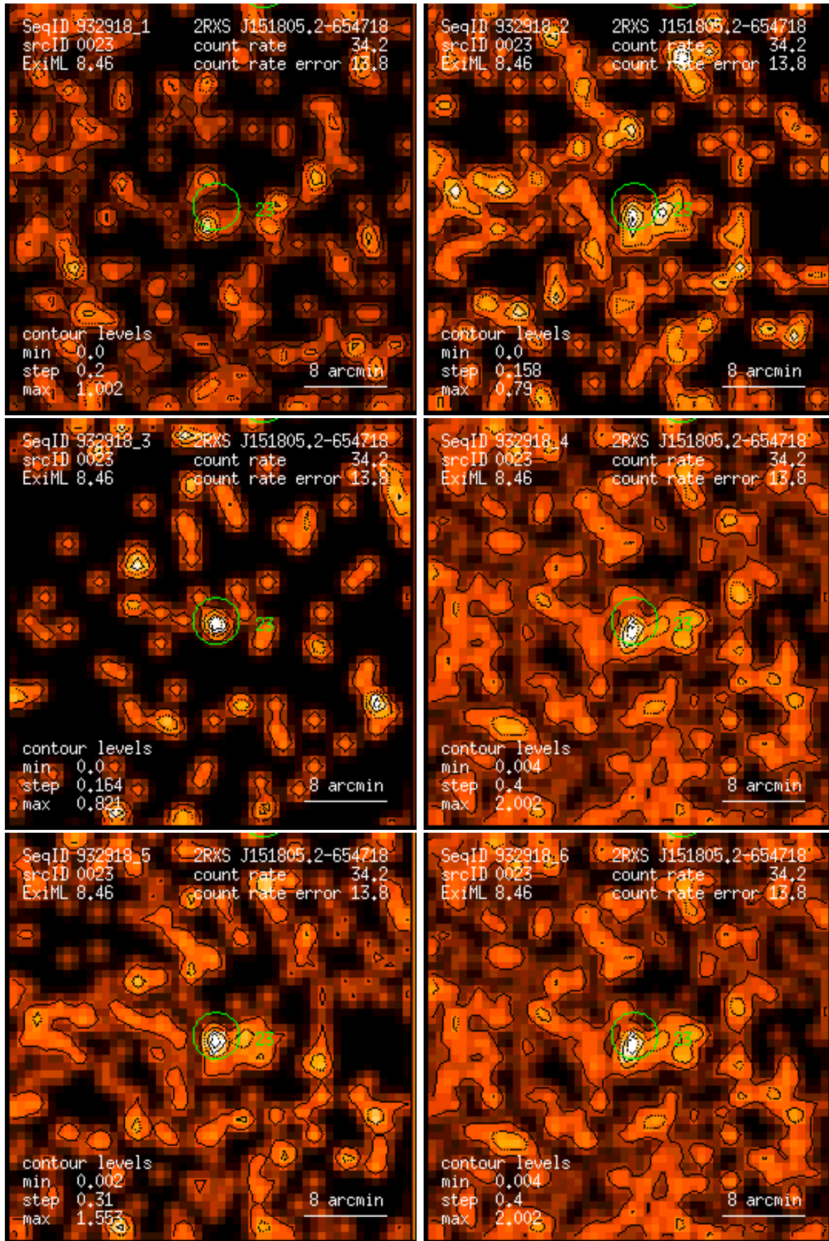
Figure 23: RASS 932918: detection 0023: band rate images, Gaussian filter: (1) PSPC channels 11 – 41, (2) 52 – 90, (3) 91 – 201, (4) 11 – 235, (5) 52 – 201, (6) 11 – 201. Broad band rates in counts/ks. Band rate contour levels in counts/ks/arcmin 2 .
