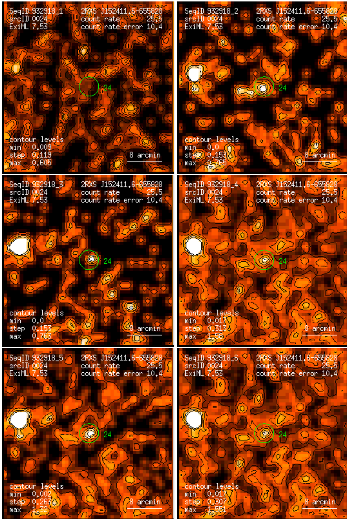
Figure 24: RASS 932918: detection 0024: band rate images, Gaussian filter: (1) PSPC channels 11 – 41, (2) 52 – 90, (3) 91 – 201, (4) 11 – 235, (5) 52 – 201, (6) 11 – 201. Broad band rates in counts/ks. Band rate contour levels in counts/ks/arcmin 2 .
