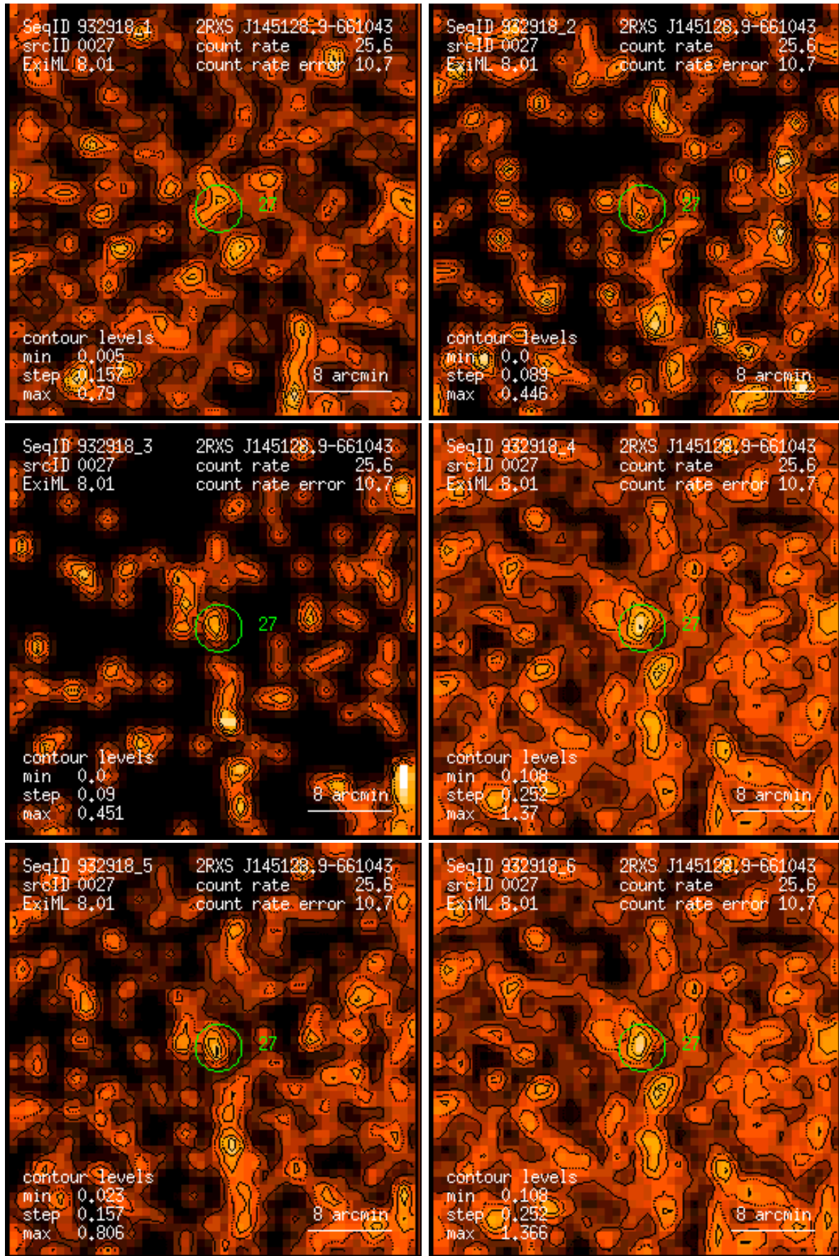
Figure 27: RASS 932918: detection 0027: band rate images, Gaussian filter: (1) PSPC channels 11 – 41, (2) 52 – 90, (3) 91 – 201, (4) 11 – 235, (5) 52 – 201, (6) 11 – 201. Broad band rates in counts/ks. Band rate contour levels in counts/ks/arcmin 2 .
