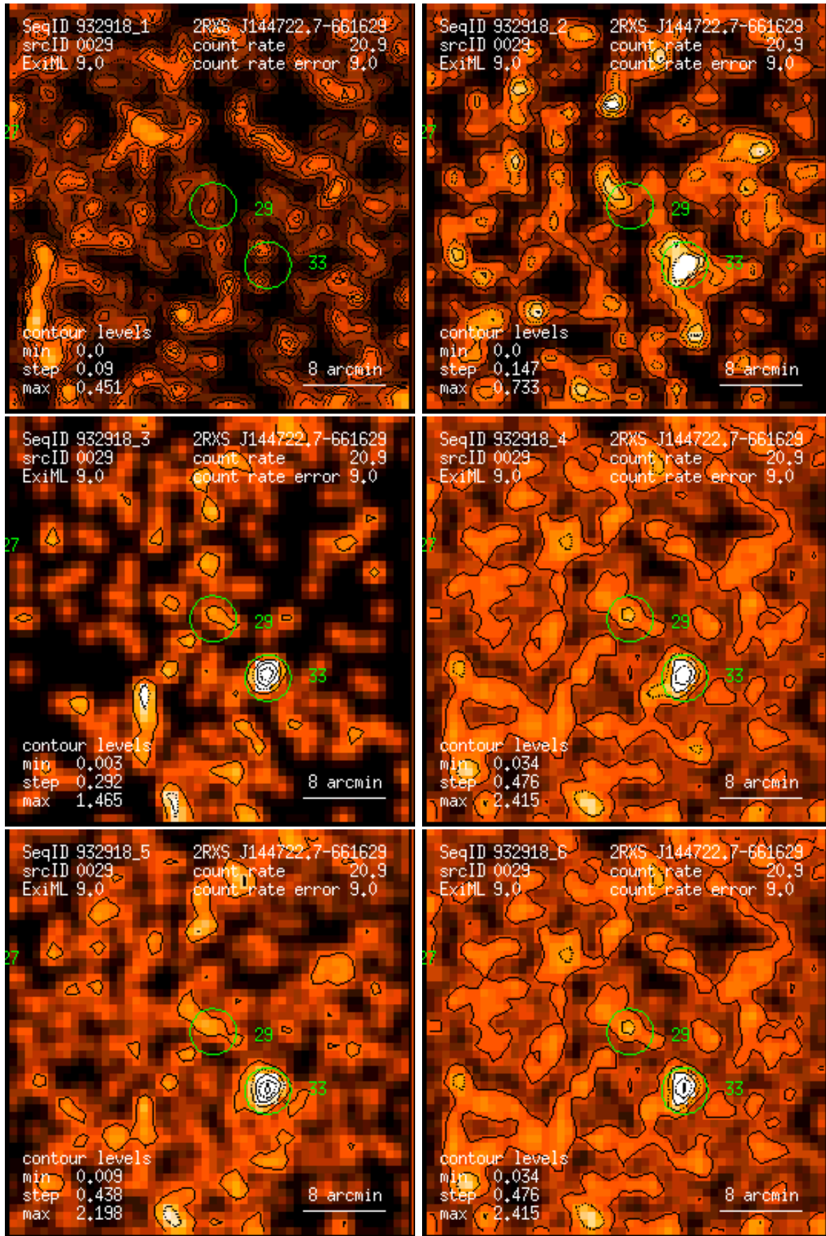
Figure 29: RASS 932918: detection 0029: band rate images, Gaussian filter: (1) PSPC channels 11 – 41, (2) 52 – 90, (3) 91 – 201, (4) 11 – 235, (5) 52 – 201, (6) 11 – 201. Broad band rates in counts/ks. Band rate contour levels in counts/ks/arcmin 2 .
