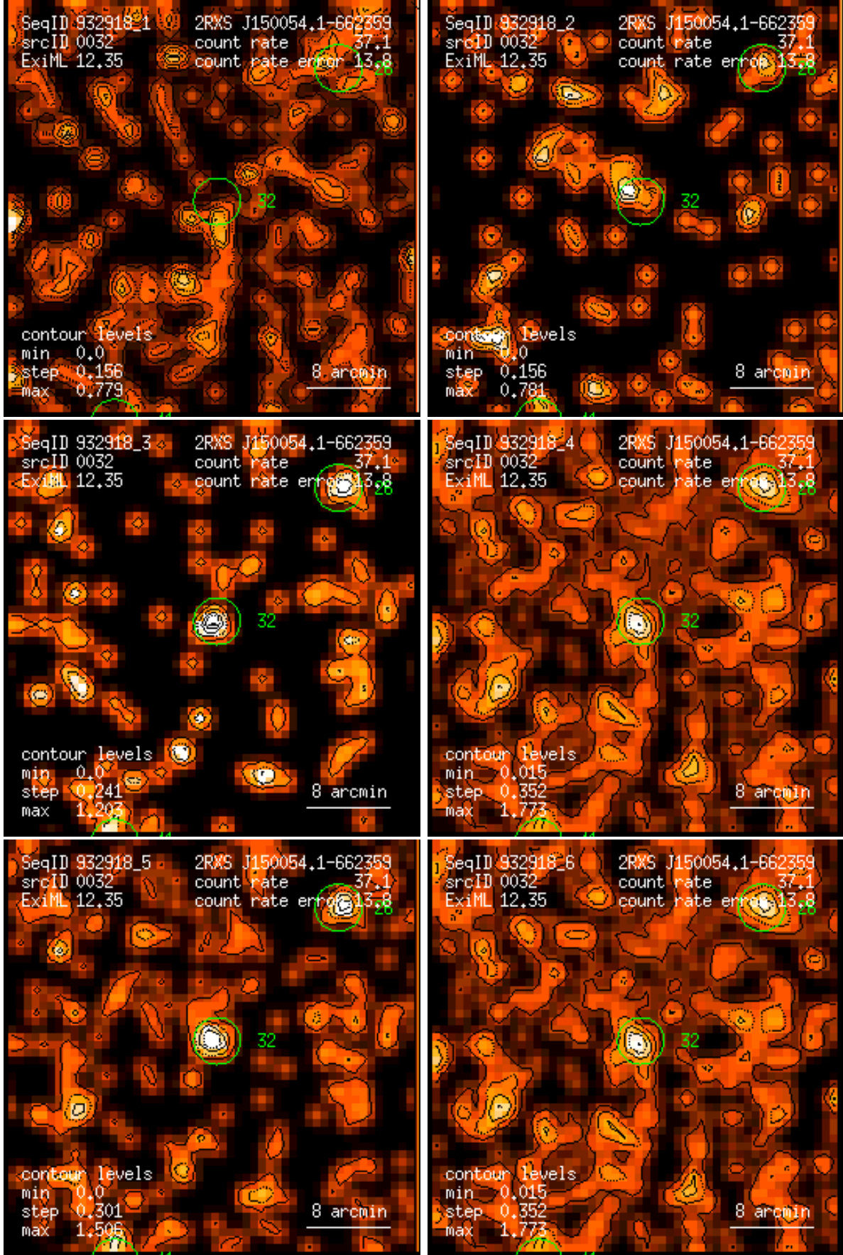
Figure 32: RASS 932918: detection 0032: band rate images, Gaussian filter: (1) PSPC channels 11 – 41, (2) 52 – 90, (3) 91 – 201, (4) 11 – 235, (5) 52 – 201, (6) 11 – 201. Broad band rates in counts/ks. Band rate contour levels in counts/ks/arcmin 2 .
