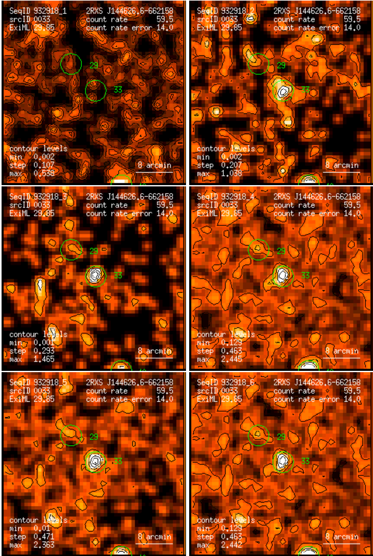
Figure 33: RASS 932918: detection 0033: band rate images, Gaussian filter: (1) PSPC channels 11 – 41, (2) 52 – 90, (3) 91 – 201, (4) 11 – 235, (5) 52 – 201, (6) 11 – 201. Broad band rates in counts/ks. Band rate contour levels in counts/ks/arcmin 2 .
