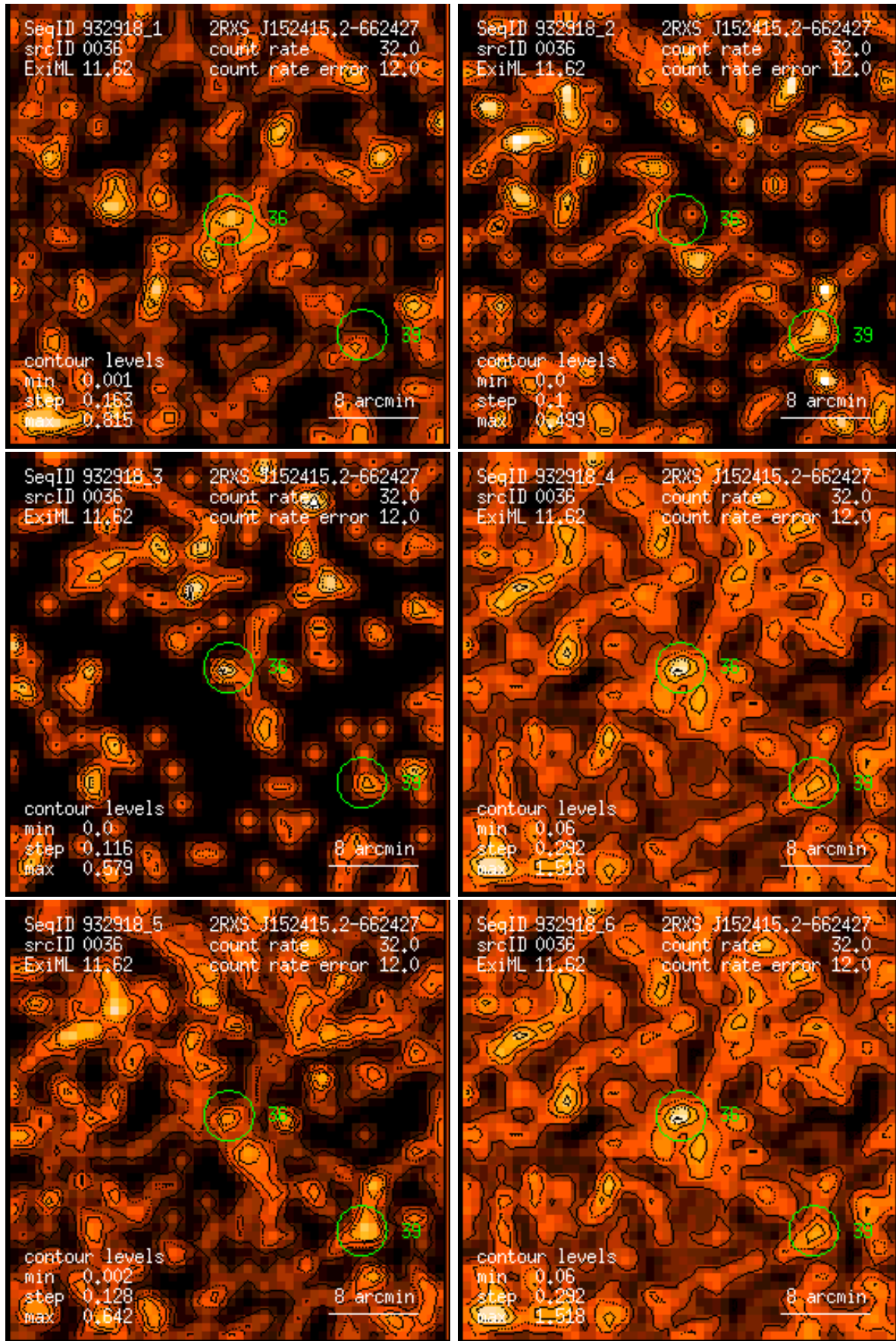
Figure 36: RASS 932918: detection 0036: band rate images, Gaussian filter: (1) PSPC channels 11 – 41, (2) 52 – 90, (3) 91 – 201, (4) 11 – 235, (5) 52 – 201, (6) 11 – 201. Broad band rates in counts/ks. Band rate contour levels in counts/ks/arcmin 2 .
