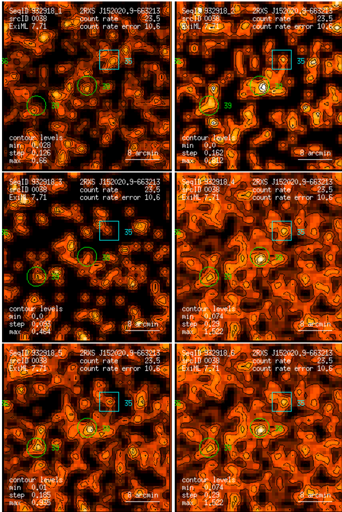
Figure 38: RASS 932918: detection 0038: band rate images, Gaussian filter: (1) PSPC channels 11 – 41, (2) 52 – 90, (3) 91 – 201, (4) 11 – 235, (5) 52 – 201, (6) 11 – 201. Broad band rates in counts/ks. Band rate contour levels in counts/ks/arcmin 2 .
