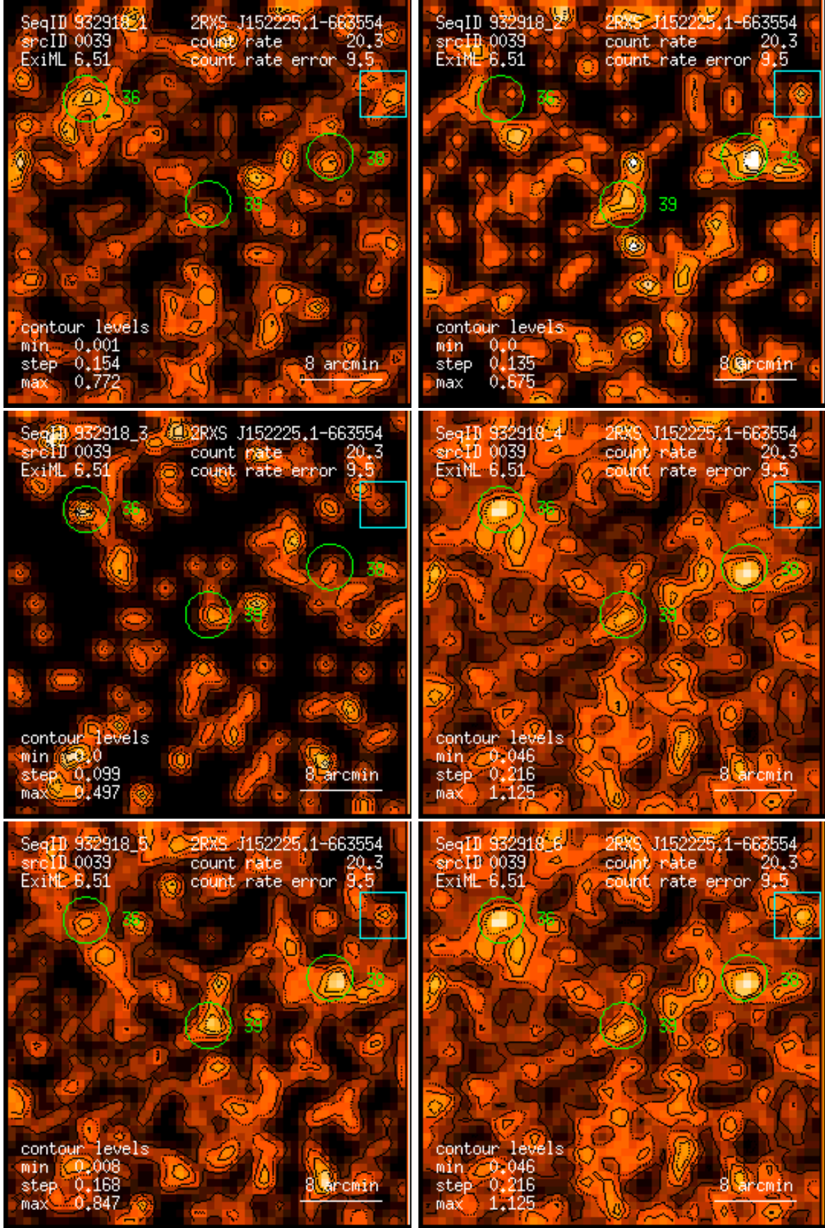
Figure 39: RASS 932918: detection 0039: band rate images, Gaussian filter: (1) PSPC channels 11 – 41, (2) 52 – 90, (3) 91 – 201, (4) 11 – 235, (5) 52 – 201, (6) 11 – 201. Broad band rates in counts/ks. Band rate contour levels in counts/ks/arcmin 2 .
