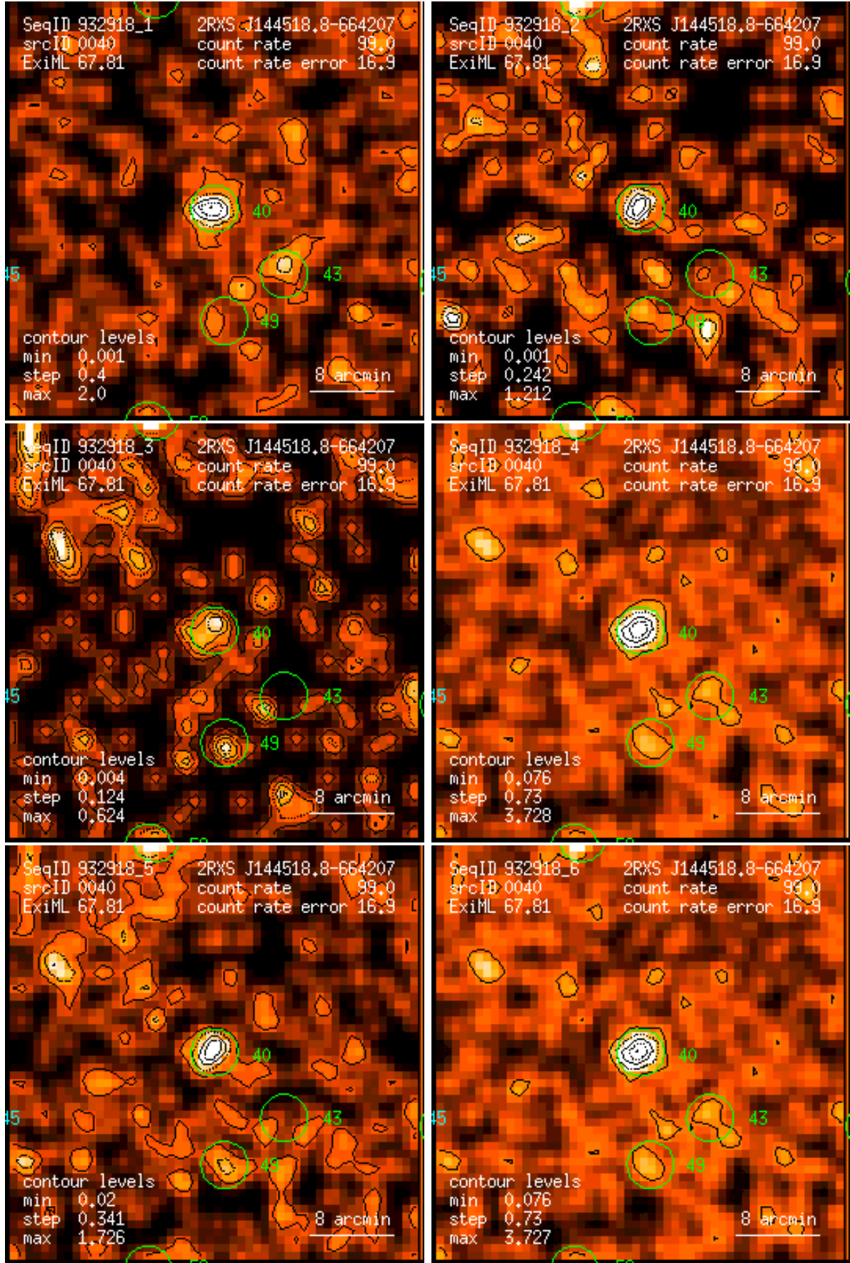
Figure 40: RASS 932918: detection 0040: band rate images, Gaussian filter: (1) PSPC channels 11 – 41, (2) 52 – 90, (3) 91 – 201, (4) 11 – 235, (5) 52 – 201, (6) 11 – 201. Broad band rates in counts/ks. Band rate contour levels in counts/ks/arcmin 2 .
