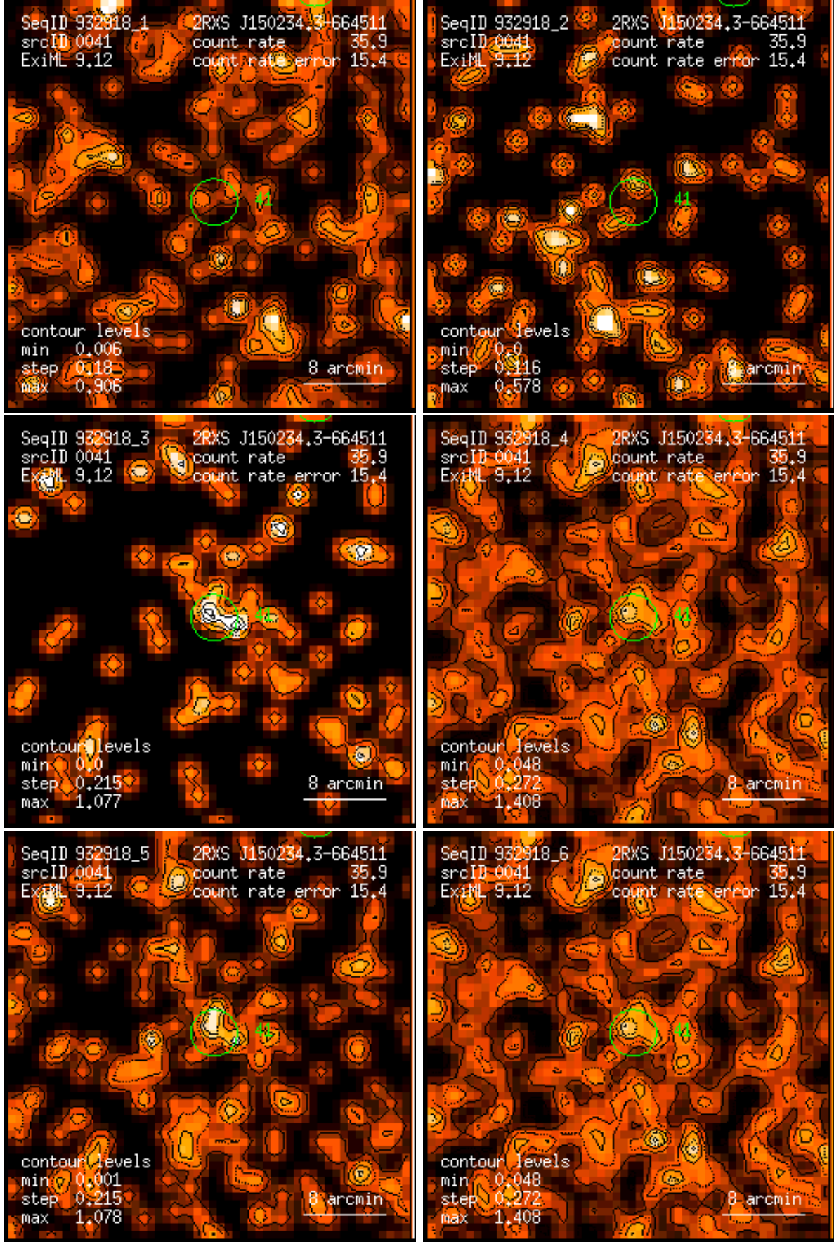
Figure 41: RASS 932918: detection 0041: band rate images, Gaussian filter: (1) PSPC channels 11 – 41, (2) 52 – 90, (3) 91 – 201, (4) 11 – 235, (5) 52 – 201, (6) 11 – 201. Broad band rates in counts/ks. Band rate contour levels in counts/ks/arcmin 2 .
