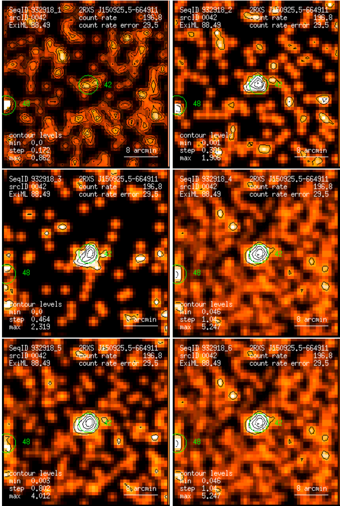
Figure 42: RASS 932918: detection 0042: band rate images, Gaussian filter: (1) PSPC channels 11 – 41, (2) 52 – 90, (3) 91 – 201, (4) 11 – 235, (5) 52 – 201, (6) 11 – 201. Broad band rates in counts/ks. Band rate contour levels in counts/ks/arcmin 2 .
